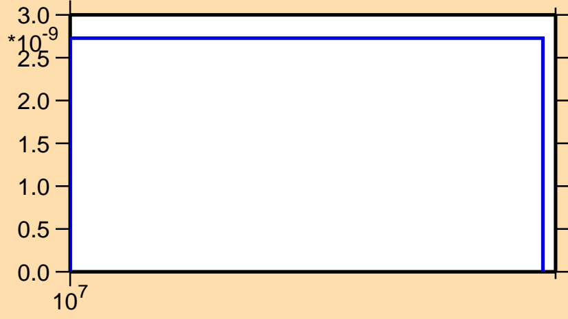
\sigma vs. E for ^{233}\text{Pa}(n,2np)
