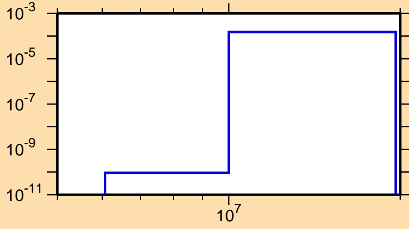
\sigma vs. E for ^{233}\text{Pa}(n,np)
