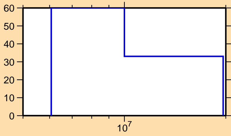
\Delta\sigma/\sigma vs. E for ^{233}\text{Pa}(n,2n)
