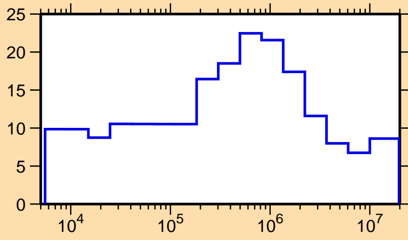
\Delta\sigma/\sigma vs. E for ^{233}\text{Pa}(n,\text{tot.})
