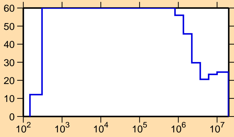
\Delta\sigma/\sigma vs. E for ^{233}\text{Pa}(n,\text{nonel.})
