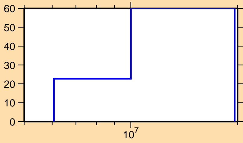
\Delta\sigma/\sigma vs. E for ^{233}\text{Pa}(n,\text{inel.})
