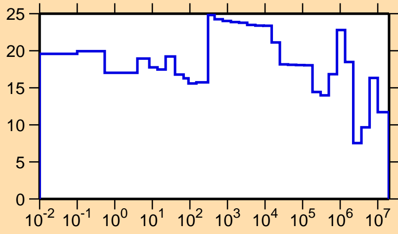
\Delta\sigma/\sigma vs. E for ^{233}\text{Pa}(n,\text{el.})
