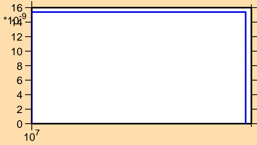
\sigma vs. E for ^{233}\text{Pa}(n,\text{nd})
