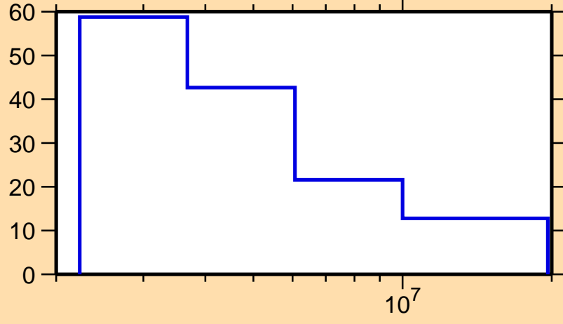
\Delta\sigma/\sigma vs. E for ^{233}\text{Pa}(n,n\text{cont.})
