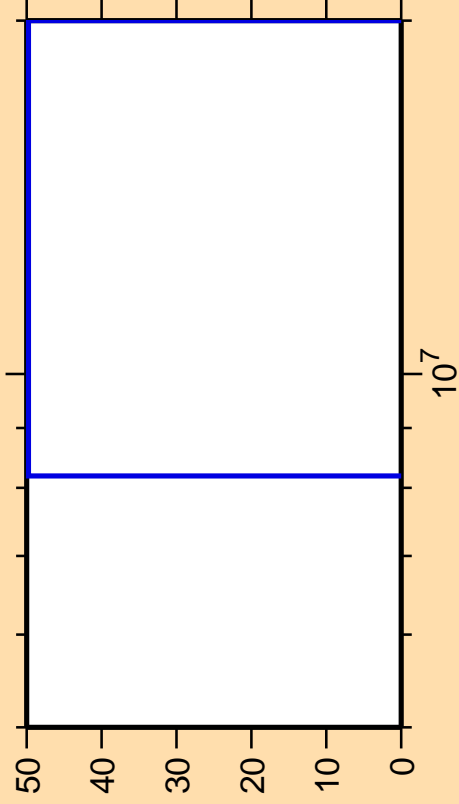
\Delta\sigma/\sigma vs. E for ^{233}\text{Pa}(n,nd)
