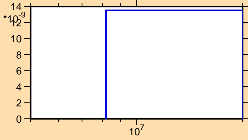
\sigma vs. E for ^{233}\text{Pa}(n,nd)
