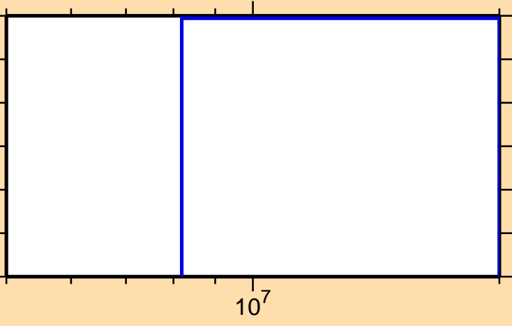
\sigma vs. E for ^{233}\text{Pa}(n,3n\alpha)
