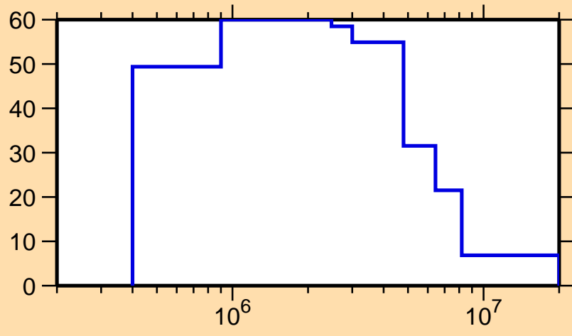
\Delta\sigma/\sigma vs. E for ^{233}\text{Pa}(n,n\text{cont.})
