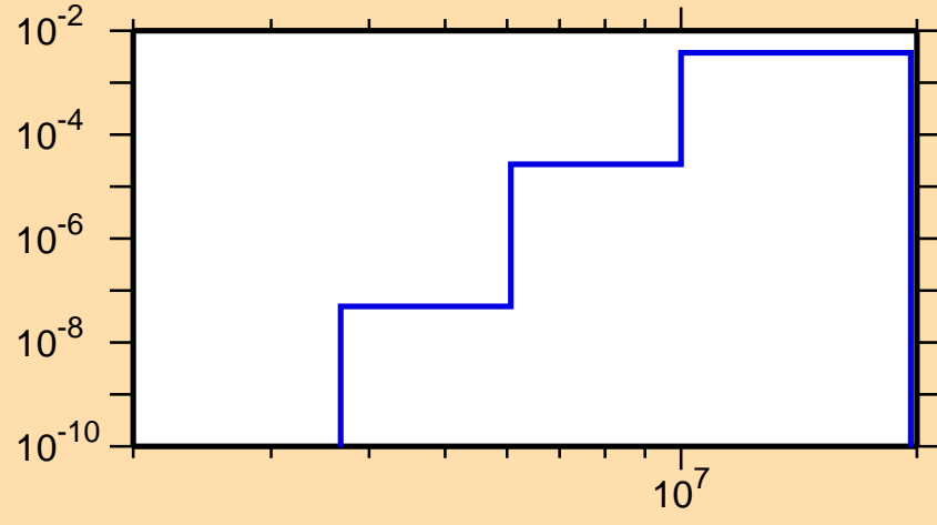
\sigma vs. E for ^{234}\text{Pa}(n,p)
