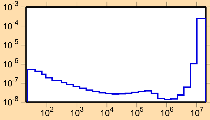
\sigma vs. E for ^{234}\text{Pa}(n,\alpha)
