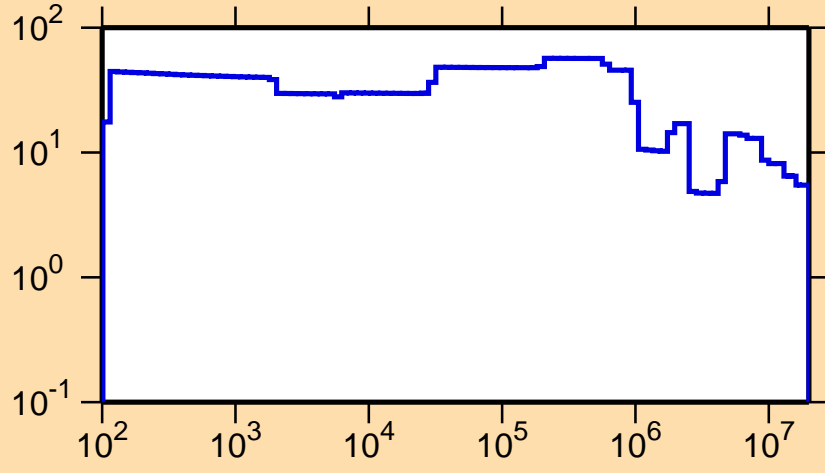
\Delta\sigma/\sigma vs. E for ^{235}\text{Pa}(n,\text{tot.})
