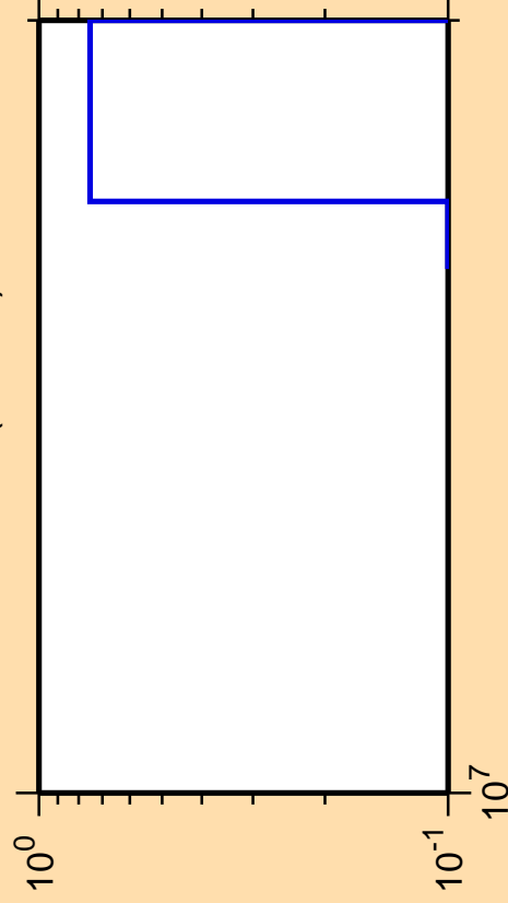
\Delta\sigma/\sigma vs. E for ^{235}\text{Pa}(n,\text{He3})
