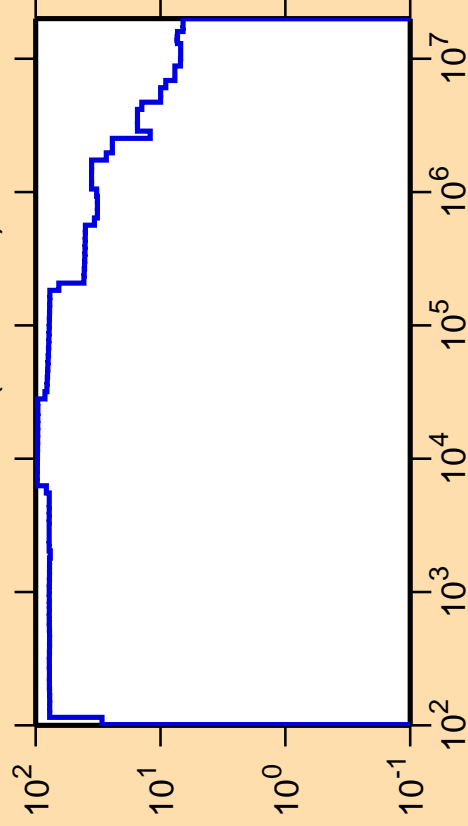
\Delta\sigma/\sigma vs. E for ^{235}\text{Pa}(n,\text{nonel.})
