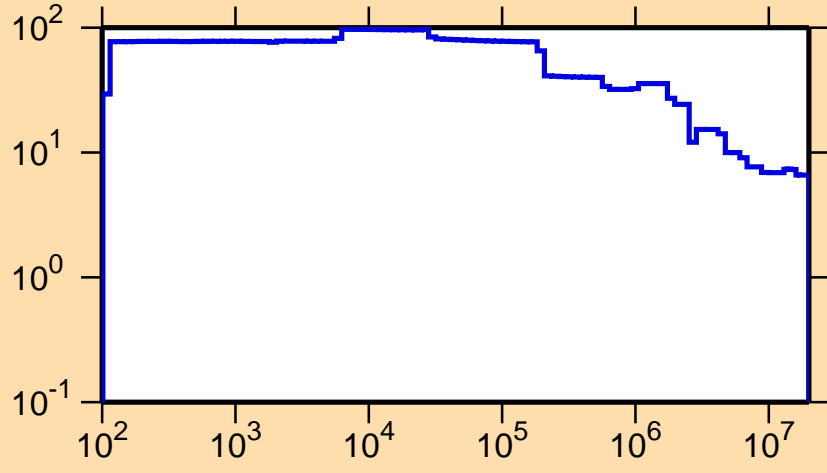
\Delta\sigma/\sigma vs. E for ^{235}\text{Pa}(n,\text{nonel.})
