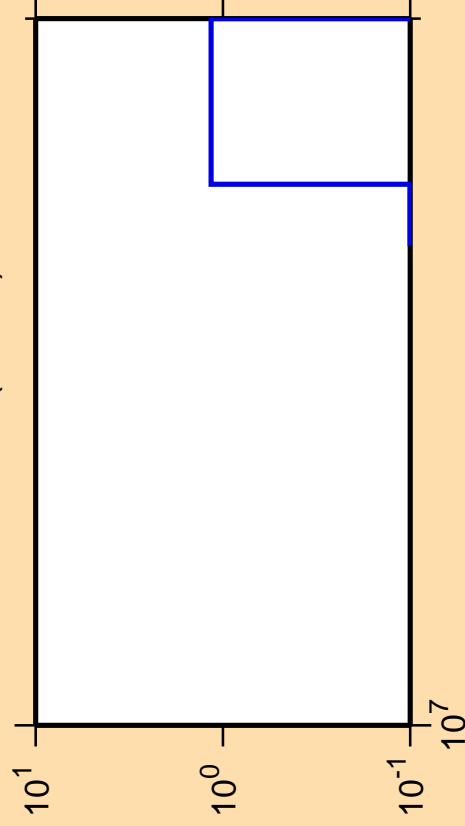
\Delta\sigma/\sigma vs. E for ^{235}\text{Pa} (mt 42)
