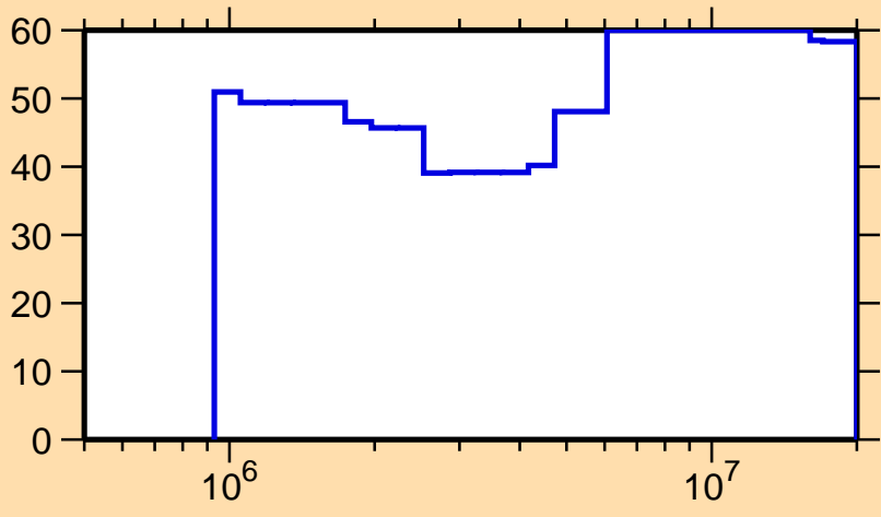
\Delta\sigma/\sigma vs. E for ^{235}\text{Pa}(n,n\text{cont.})
