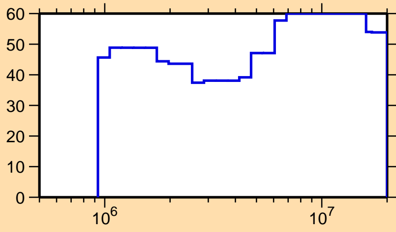
\Delta\sigma/\sigma vs. E for ^{235}\text{Pa}(n,\text{inel.})
