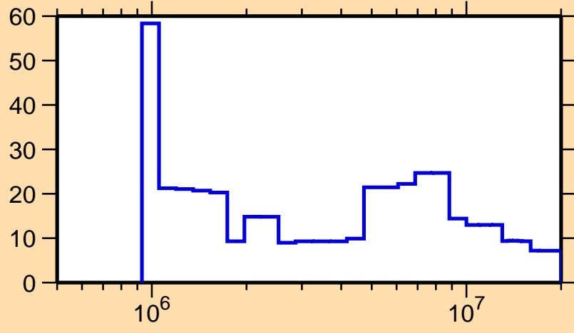
\Delta\sigma/\sigma vs. E for ^{235}\text{Pa}(n,\text{el.})
