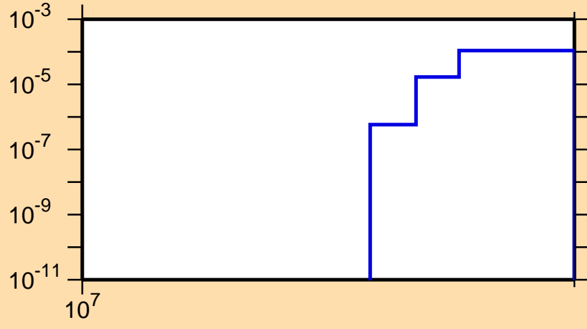
\sigma vs. E for ^{235}\text{Pa}(n,3n\alpha)
