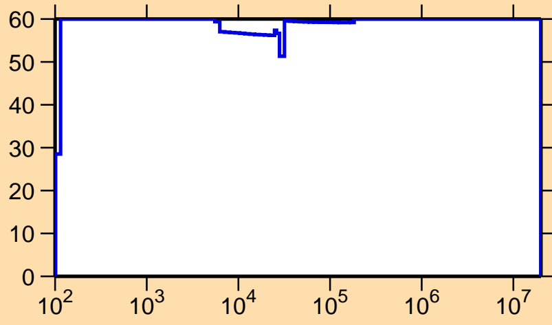
\Delta\sigma/\sigma vs. E for ^{235}\text{Pa}(n,\gamma)
