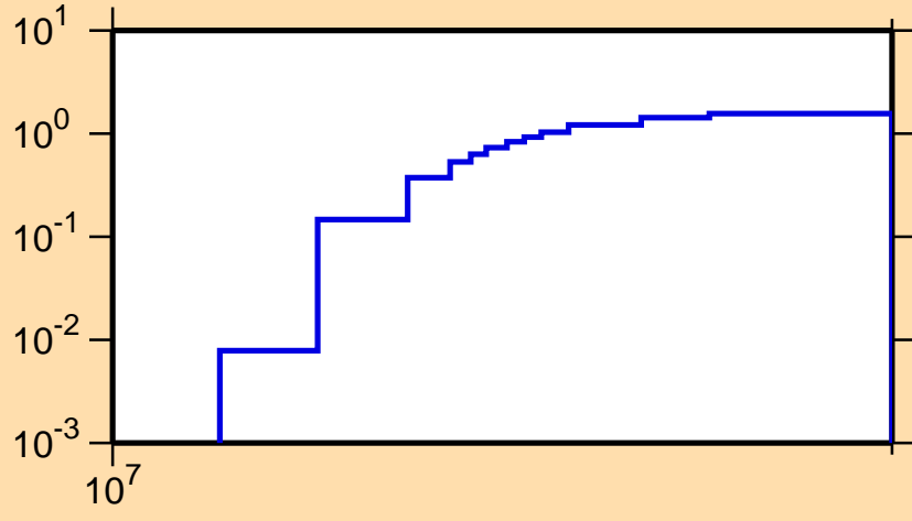
\sigma vs. E for ^{235}\text{Pa}(n,3n)
