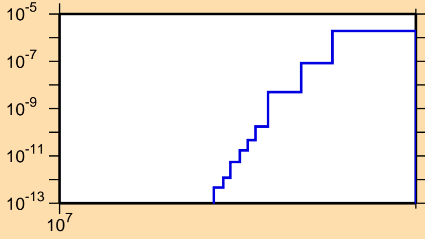
\sigma vs. E for ^{235}\text{Pa}(n,\text{nd})
