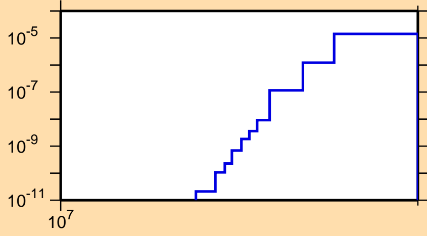
\sigma vs. E for ^{235}\text{Pa}(n,nt)
