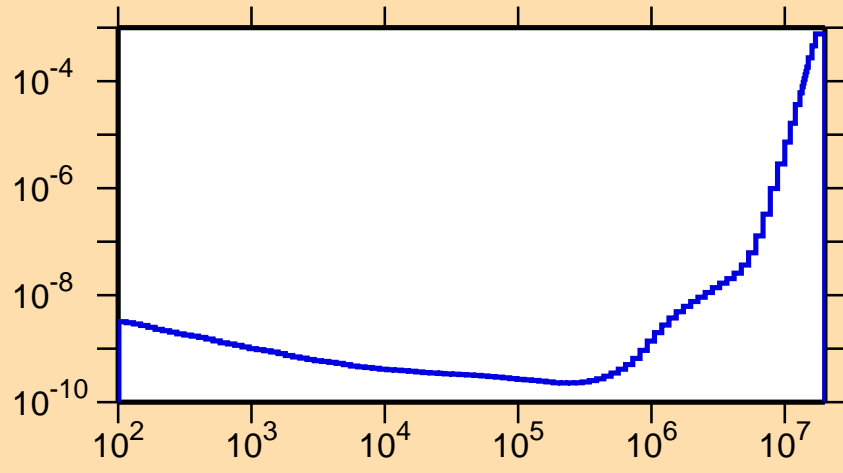
\sigma vs. E for ^{235}\text{Pa}(n,\alpha)
