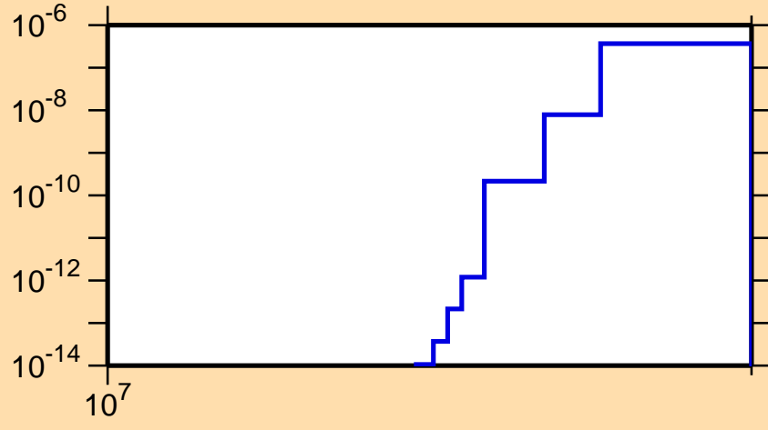
\sigma vs. E for ^{235}\text{Pa}(n,2np)
