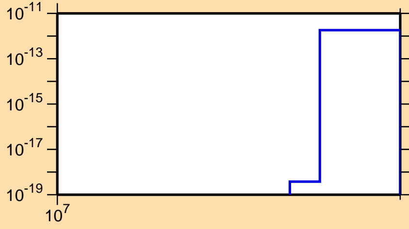
\sigma vs. E for ^{235}\text{Pa}(\text{mt } 11)
