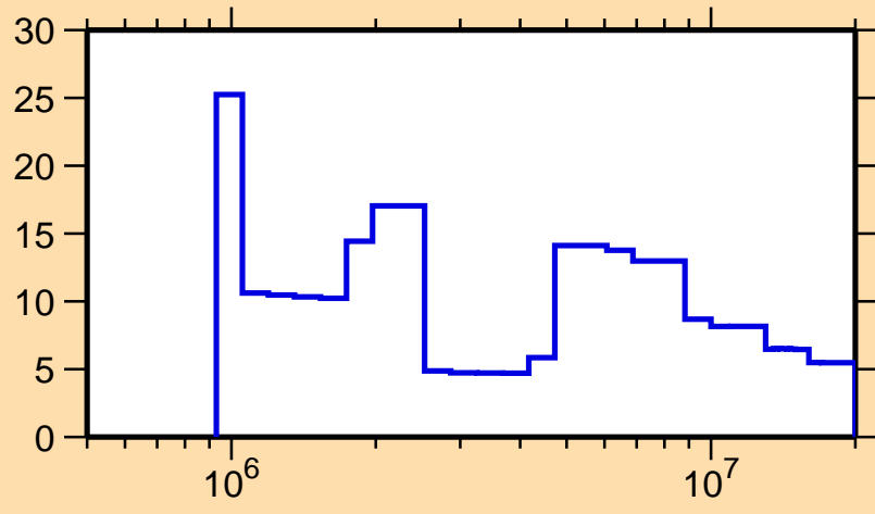
\Delta\sigma/\sigma vs. E for ^{235}\text{Pa}(n, \text{tot.})
