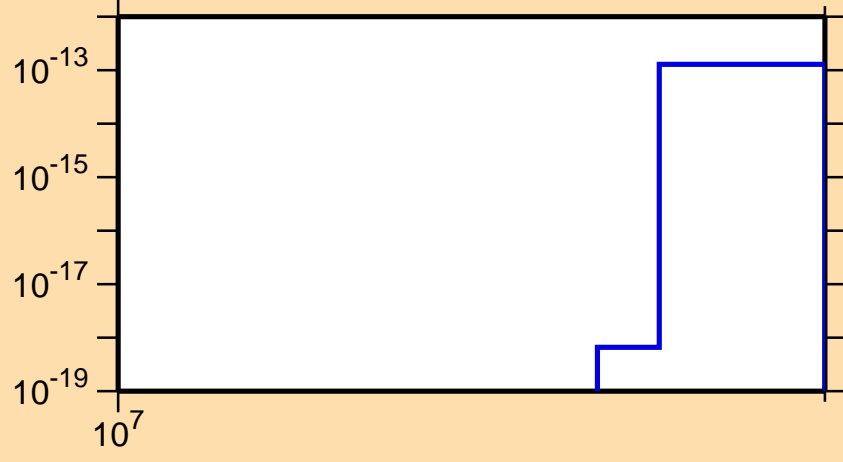
\sigma vs. E for ^{235}\text{Pa} (mt 42)
