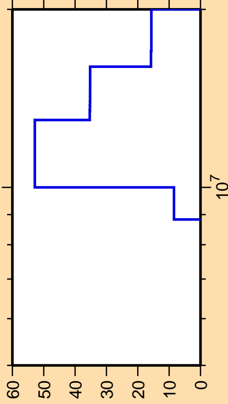
\Delta\sigma/\sigma vs. E for ^{235}\text{Pa}(n,t)
