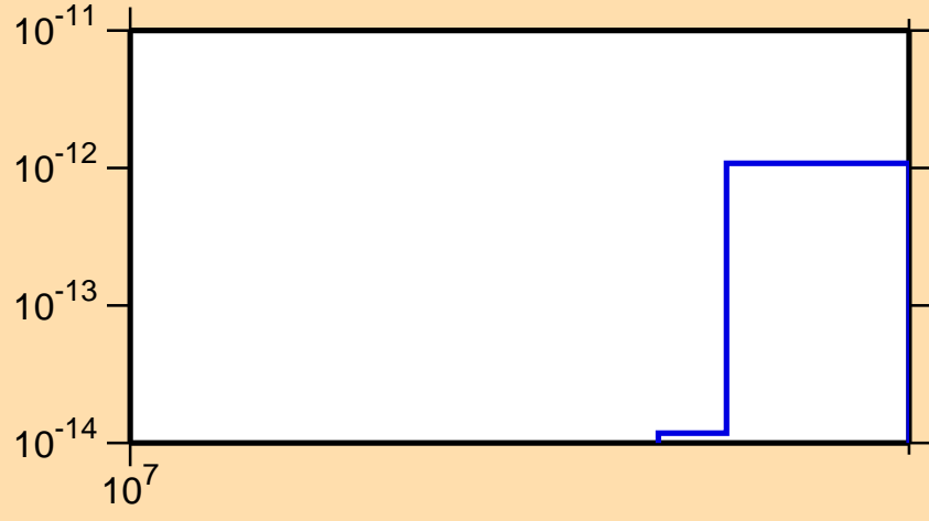
\sigma vs. E for ^{235}\text{Pa}(n,\text{He3})
