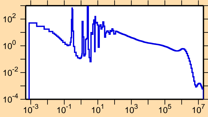
\sigma vs. E for ^{235}\text{Pa}(n,\gamma)
