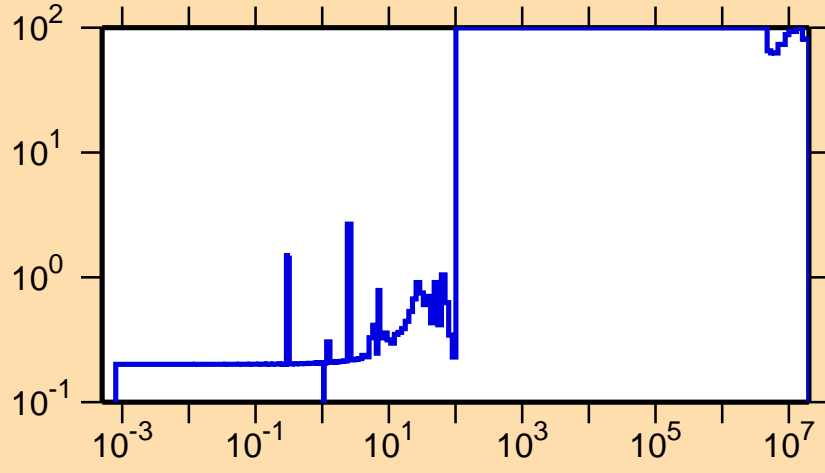
\Delta\sigma/\sigma vs. E for ^{235}\text{Pa}(n,f)
