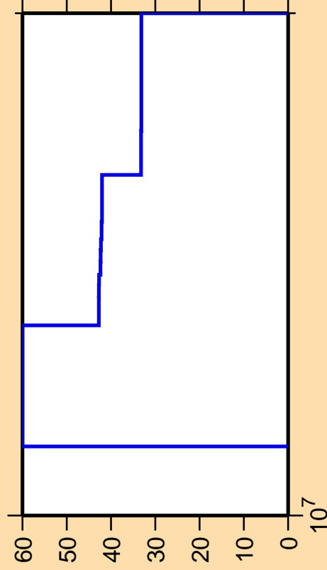
\Delta\sigma/\sigma vs. E for ^{235}\text{Pa}(n,3n)
