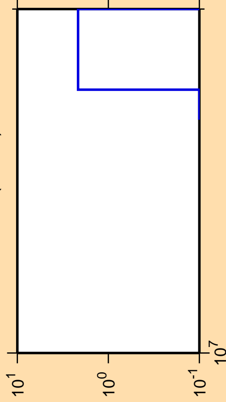
\Delta\sigma/\sigma vs. E for ^{235}\text{Pa}(\text{mt } 11)
