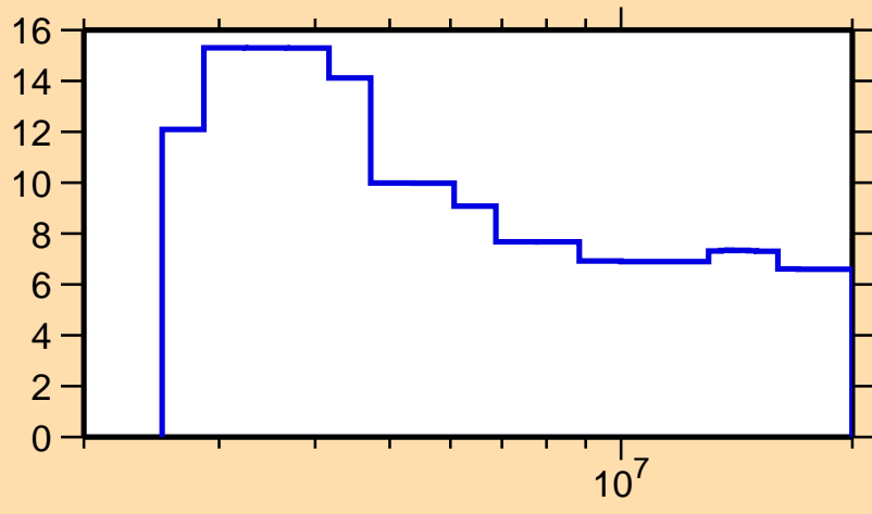
\Delta\sigma/\sigma vs. E for ^{235}\text{Pa}(n,\text{nonel.})
