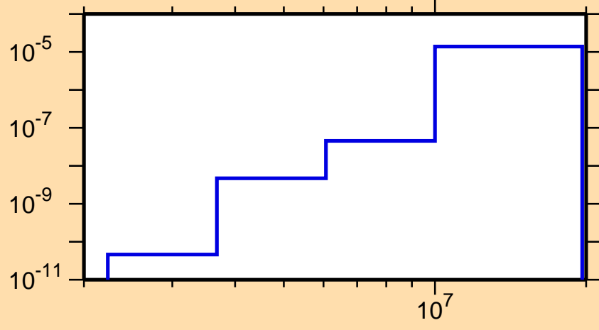
\sigma vs. E for ^{235}\text{Pa}(n,n\alpha)
