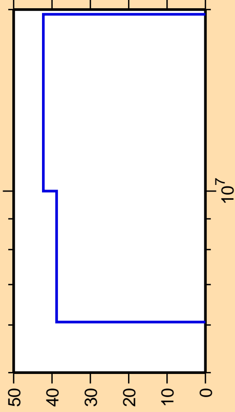
\Delta\sigma/\sigma vs. E for ^{235}\text{Pa}(n,2n)
