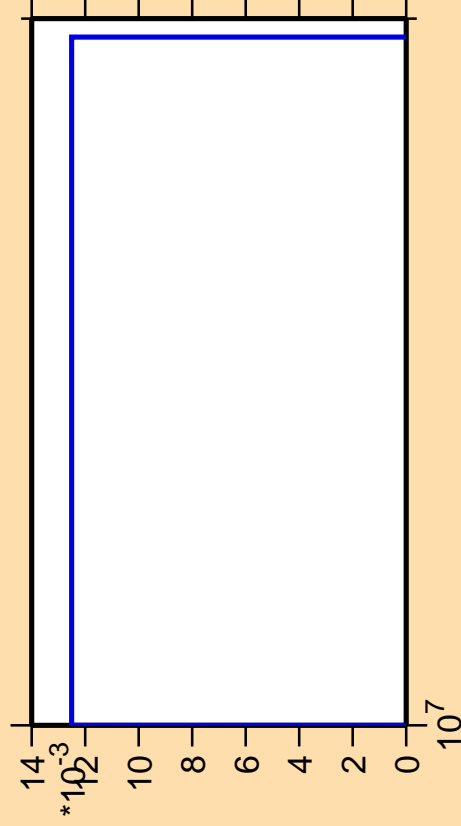
\Delta\sigma/\sigma vs. E for ^{235}\text{Pa} (mt 11)
