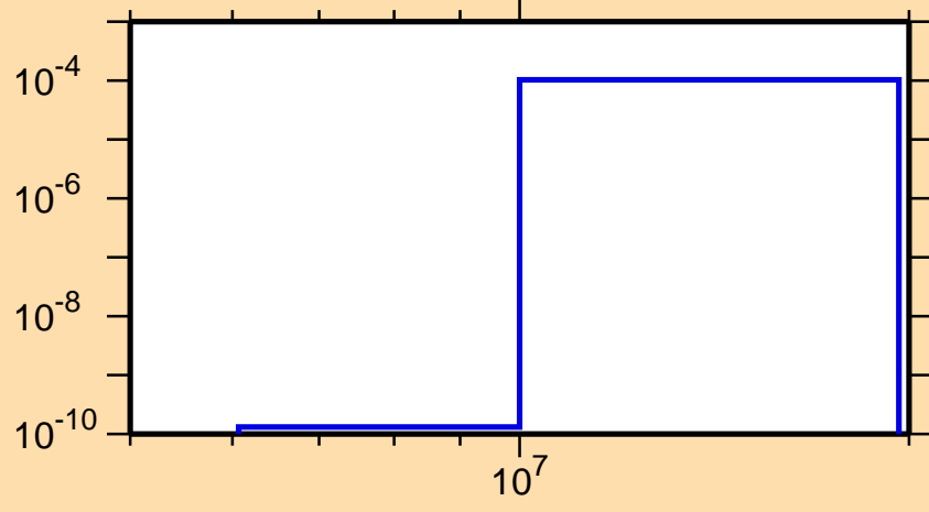
\sigma vs. E for ^{235}\text{Pa}(n,d)
