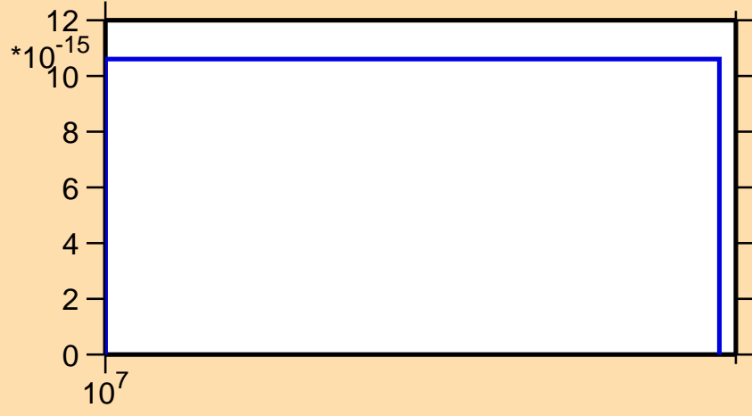
\sigma vs. E for ^{235}\text{Pa} (mt 11)
