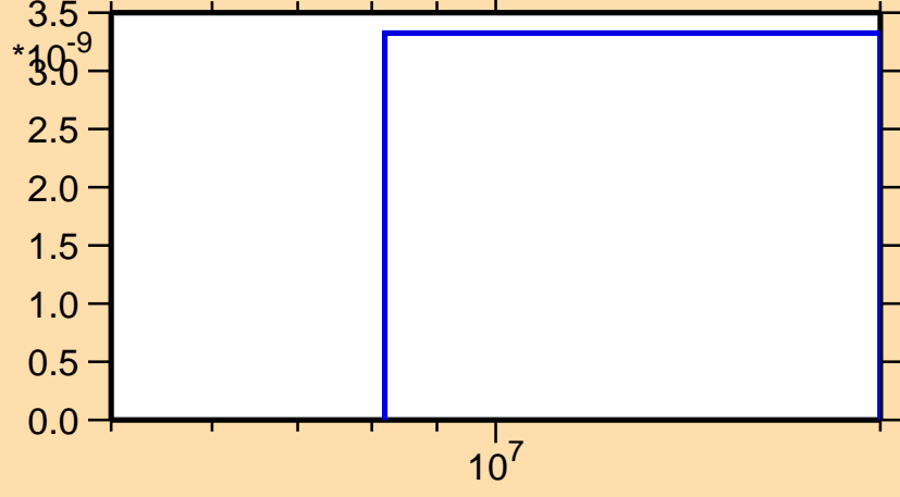
\sigma vs. E for ^{235}\text{Pa}(n,2np)
