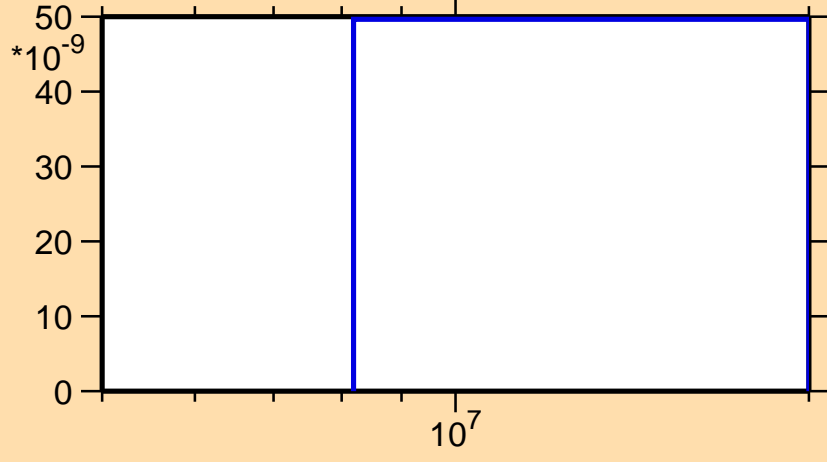
\sigma vs. E for ^{235}\text{Pa}(n,2n\alpha)
