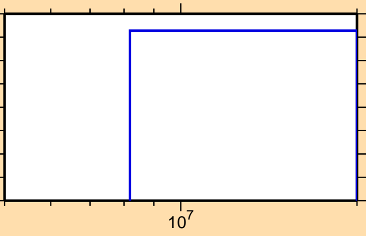
\sigma vs. E for ^{235}\text{Pa}(n,np)
