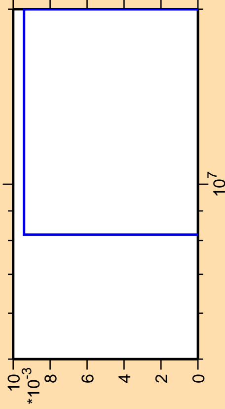
\Delta\sigma/\sigma vs. E for ^{235}\text{Pa} (mt 42)
