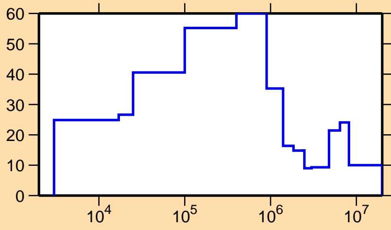
\Delta\sigma/\sigma vs. E for ^{235}\text{Pa}(n,\text{el.})
