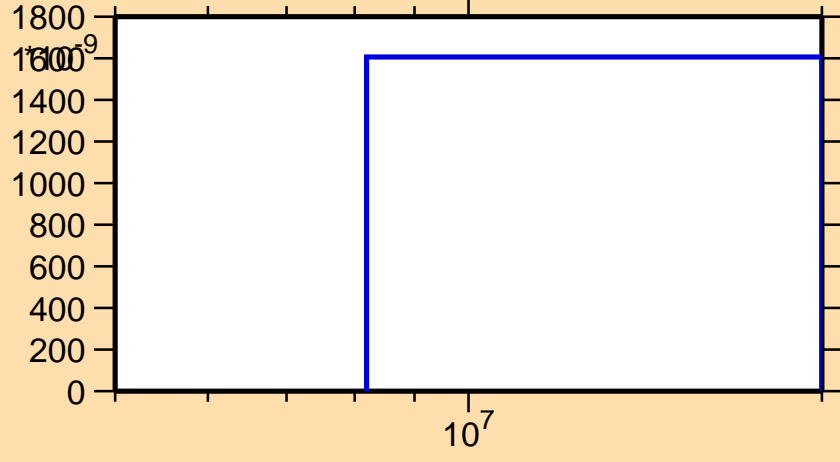
\sigma vs. E for ^{235}\text{Pa}(n,3n\alpha)
