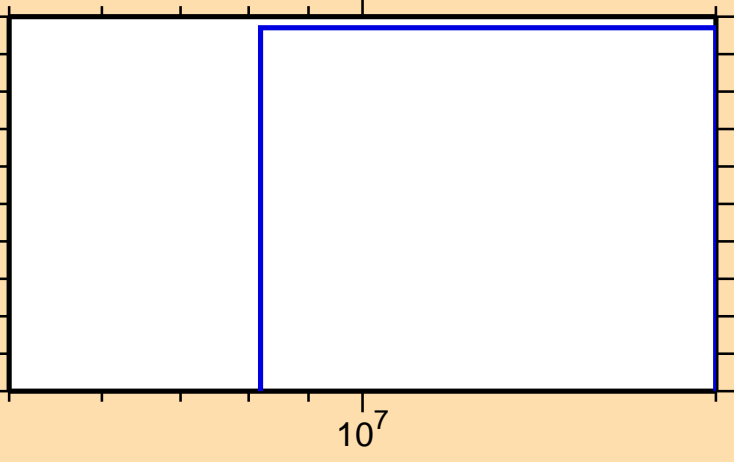
\sigma vs. E for ^{235}\text{Pa}(n,nd)
