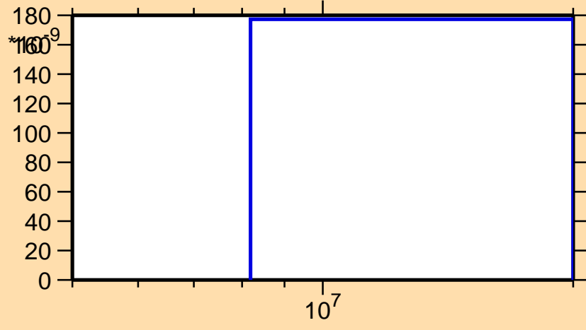
\sigma vs. E for ^{235}\text{Pa}(n,nt)
