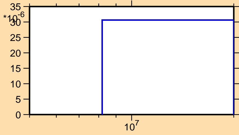
\sigma vs. E for ^{235}\text{Pa}(n,t)
