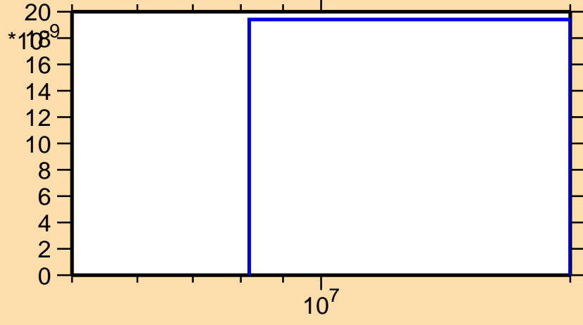
\sigma vs. E for ^{235}\text{Pa}(n,nd)
