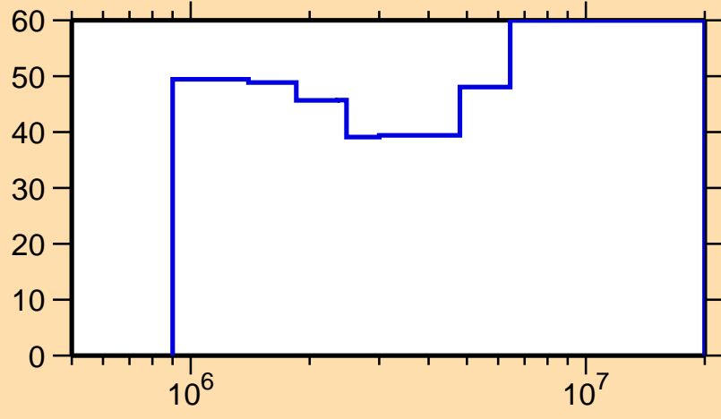
\Delta\sigma/\sigma vs. E for ^{235}\text{Pa}(n,n\text{cont.})
