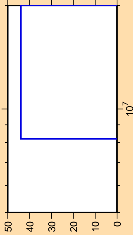
\Delta\sigma/\sigma vs. E for ^{235}\text{Pa}(n,nd)
