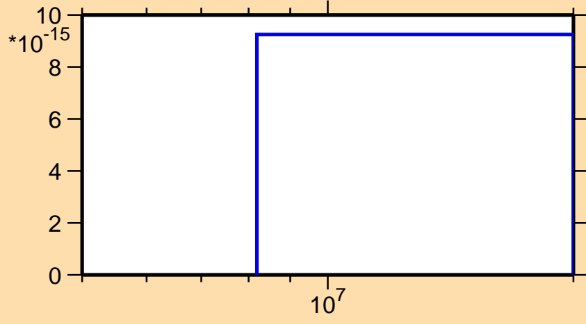
\sigma vs. E for ^{235}\text{Pa}(n,\text{He}3)
