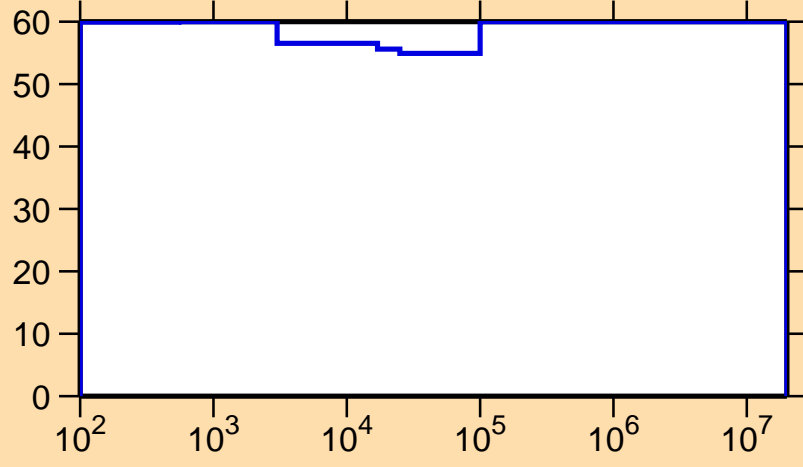
\Delta\sigma/\sigma vs. E for ^{235}\text{Pa}(n,\gamma)
