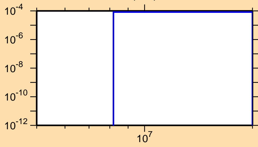
\sigma vs. E for ^{235}\text{Pa}(n,d)
