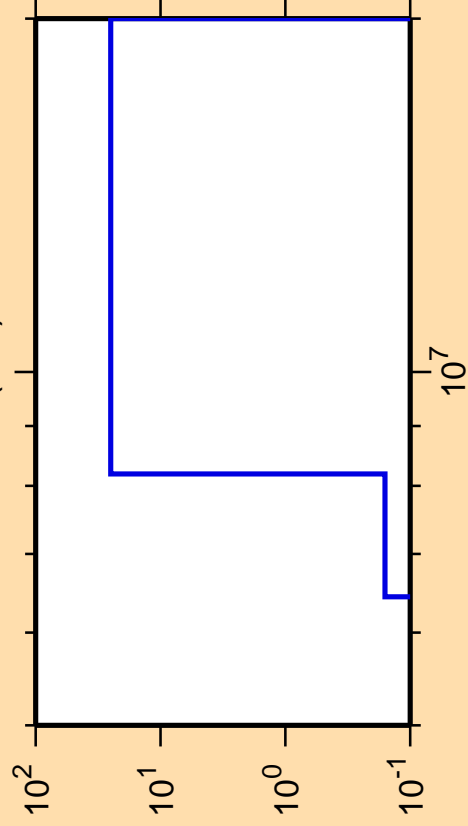
\Delta\sigma/\sigma vs. E for ^{235}\text{Pa}(n,d)
