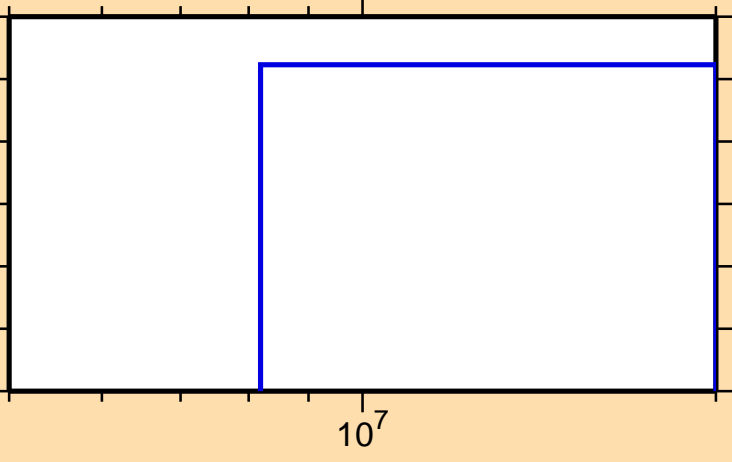
\sigma vs. E for ^{235}\text{Pa} (mt 42)
