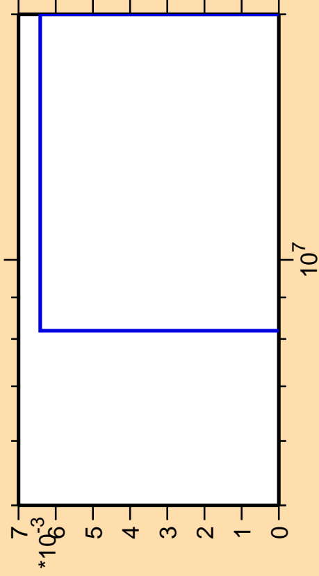
\Delta\sigma/\sigma vs. E for ^{235}\text{Pa}(n,\text{He}3)
