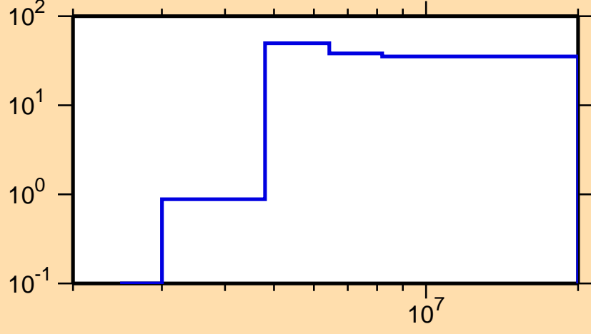
\Delta\sigma/\sigma vs. E for ^{235}\text{Pa}(n,p)
