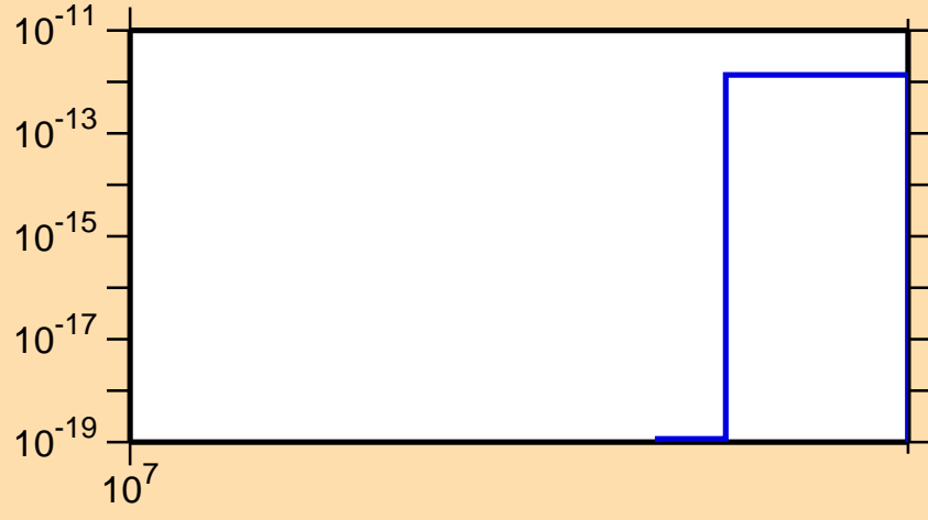
\sigma vs. E for ^{236}\text{Pa} (mt 11)
