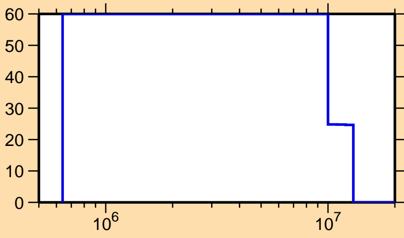
\Delta\sigma/\sigma vs. E for ^{236}\text{Pa}(n,n_1)
