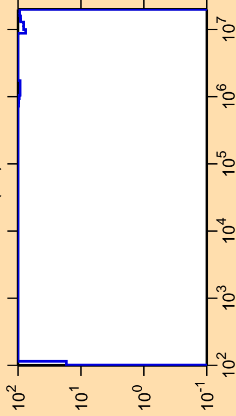
\Delta\sigma/\sigma vs. E for ^{236}\text{Pa}(n,f)
