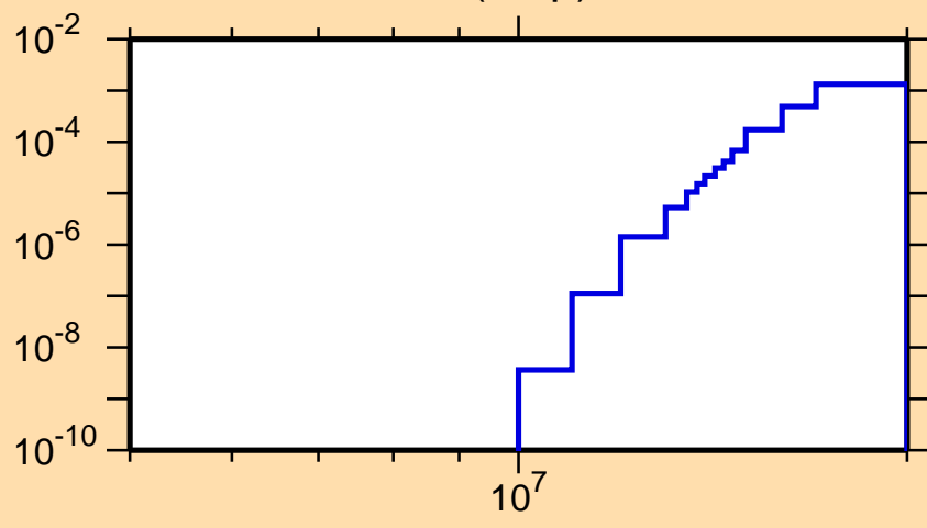
\sigma vs. E for ^{236}\text{Pa}(n,np)
