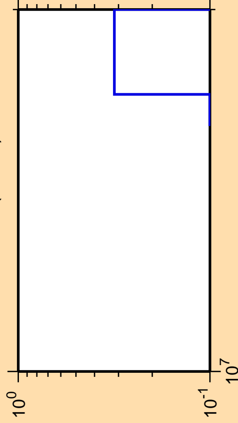
\Delta\sigma/\sigma vs. E for ^{236}\text{Pa} (mt 42)
