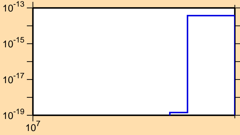
\sigma vs. E for ^{236}\text{Pa} (mt 42)
