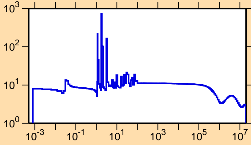
\sigma vs. E for ^{236}\text{Pa}(n,\text{el.})
