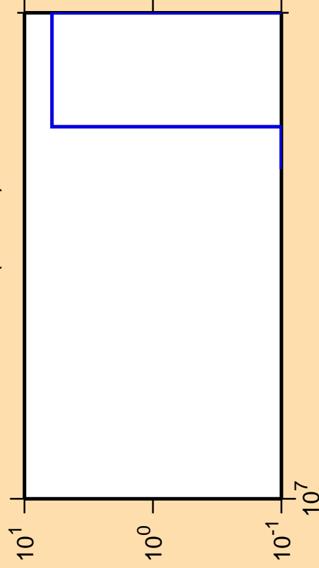
\Delta\sigma/\sigma vs. E for ^{236}\text{Pa} (mt 11)
