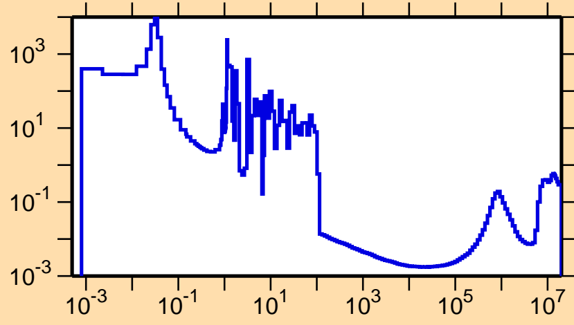
\sigma vs. E for ^{236}\text{Pa}(n,f)
