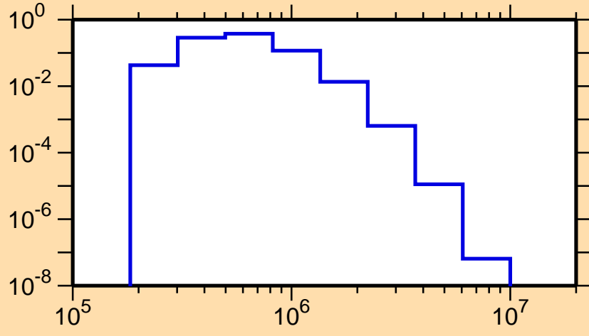
\sigma vs. E for ^{236}\text{Pa}(n,n_3)
