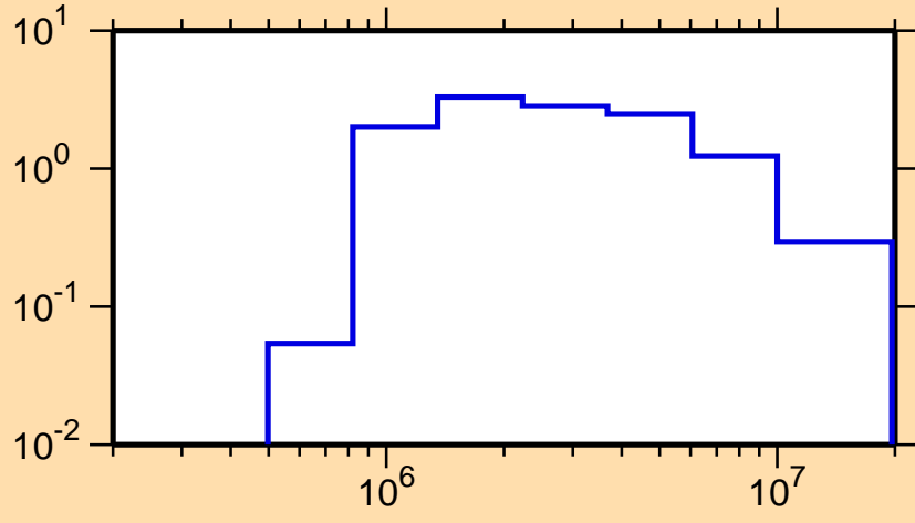
\sigma vs. E for ^{236}\text{Pa}(n,n\text{cont.})
