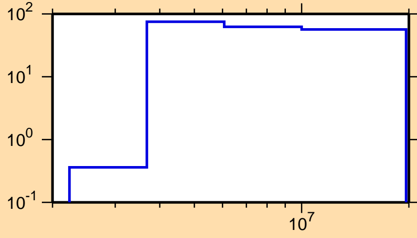
\Delta\sigma/\sigma vs. E for ^{236}\text{Pa}(n,p)
