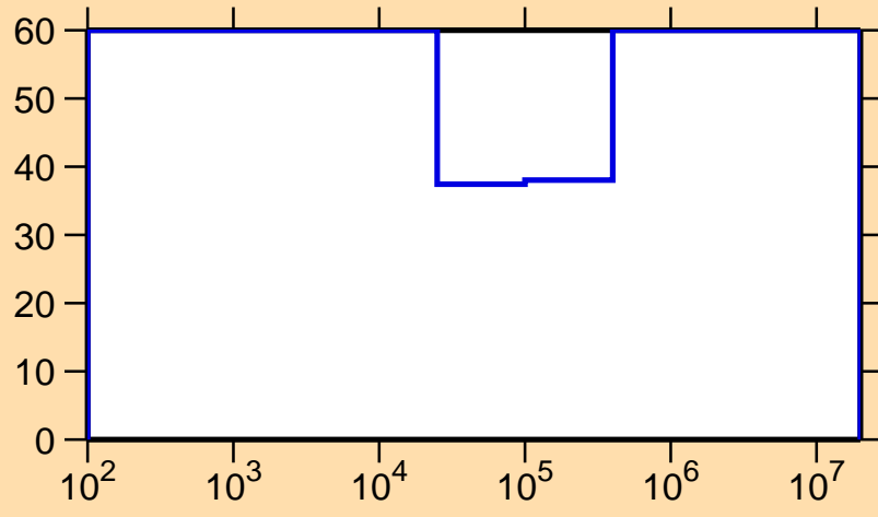
\Delta\sigma/\sigma vs. E for ^{236}\text{Pa}(n,\gamma)
