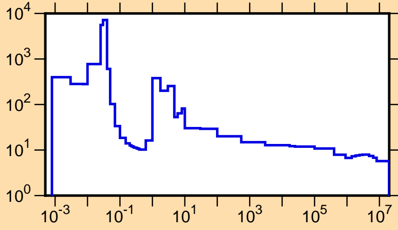
\sigma vs. E for ^{236}\text{Pa}(n,\text{tot.})
