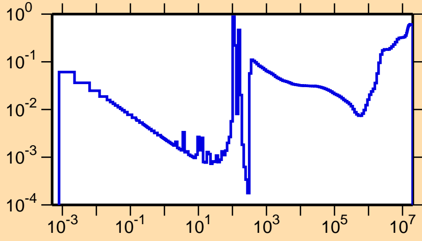
\sigma vs. E for ^{237}\text{Pa}(n,f)
