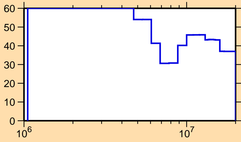
\Delta\sigma/\sigma vs. E for ^{237}\text{Pa}(n,n\text{cont.})
