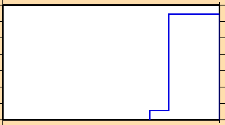
\sigma vs. E for ^{237}\text{Pa} (mt 11)
