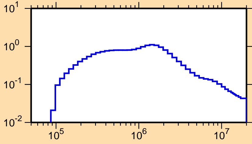
\sigma vs. E for ^{237}\text{Pa}(n,n_2)
