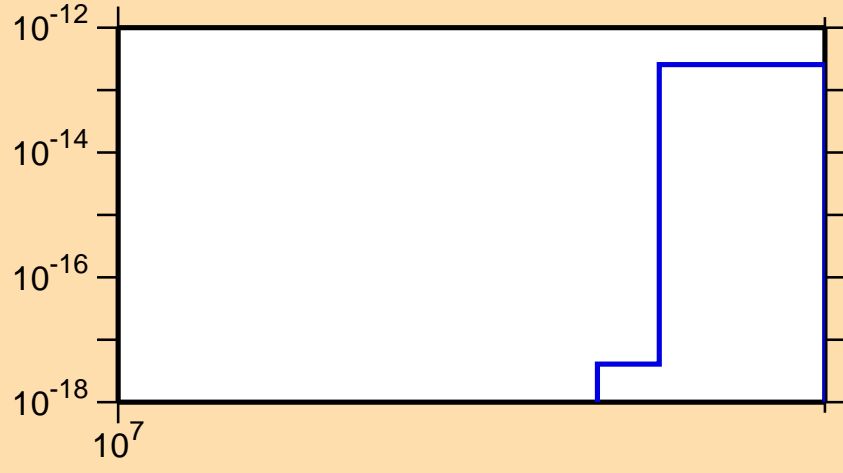
\sigma vs. E for ^{237}\text{Pa} (mt 42)
