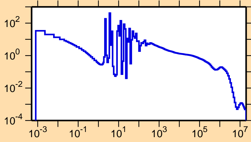
\sigma vs. E for ^{237}\text{Pa}(n,\gamma)
