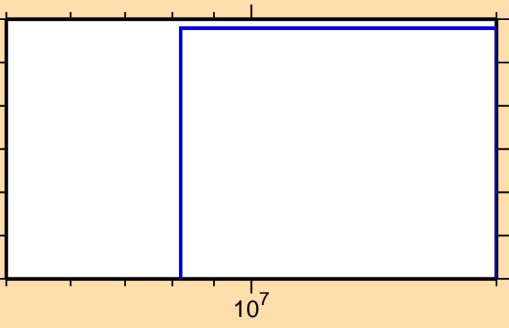
\sigma vs. E for ^{237}\text{Pa}(n,t)
