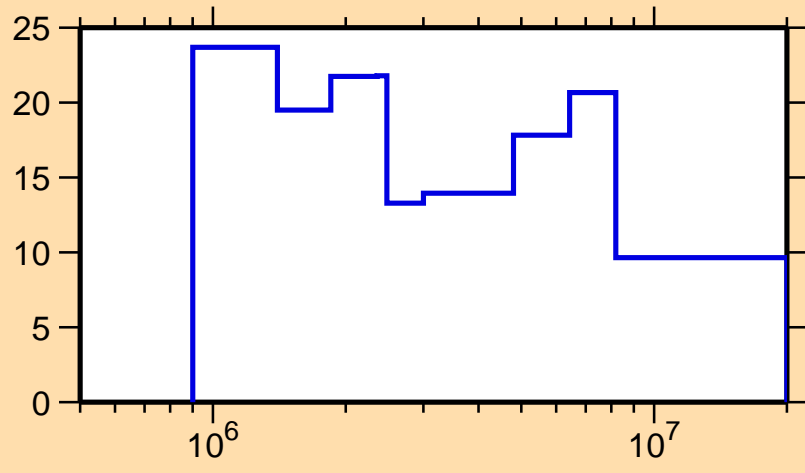
\Delta\sigma/\sigma vs. E for ^{237}\text{Pa}(n, tot.)
