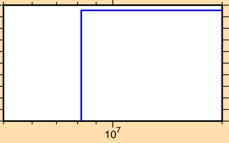
\sigma vs. E for ^{237}\text{Pa}(n,\text{nd})
