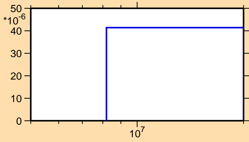
\sigma vs. E for ^{237}\text{Pa}(n,np)
