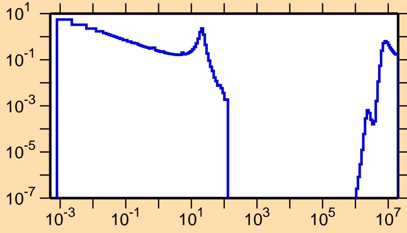
\sigma vs. E for ^{238}\text{Pa}(n,f)
