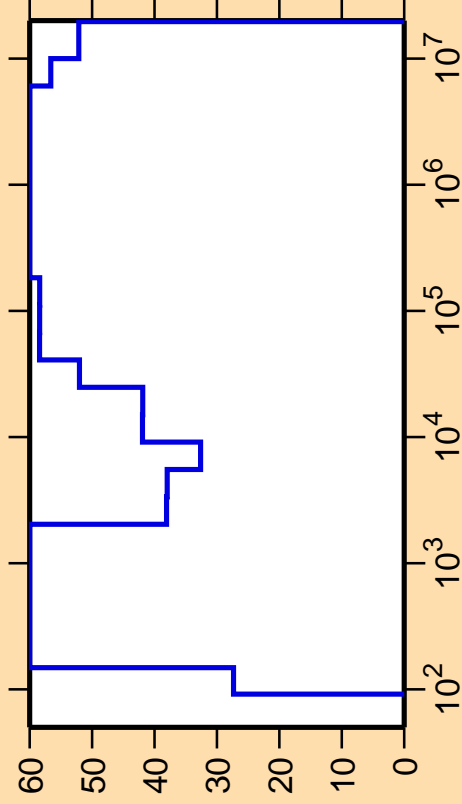
\Delta\sigma/\sigma vs. E for ^{238}\text{Pa}(n,\text{nonel.})
