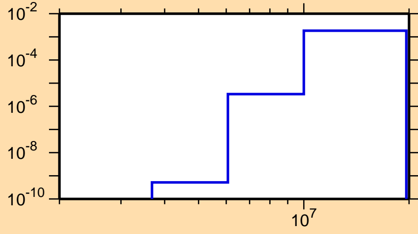
\sigma vs. E for ^{238}\text{Pa}(n,p)
