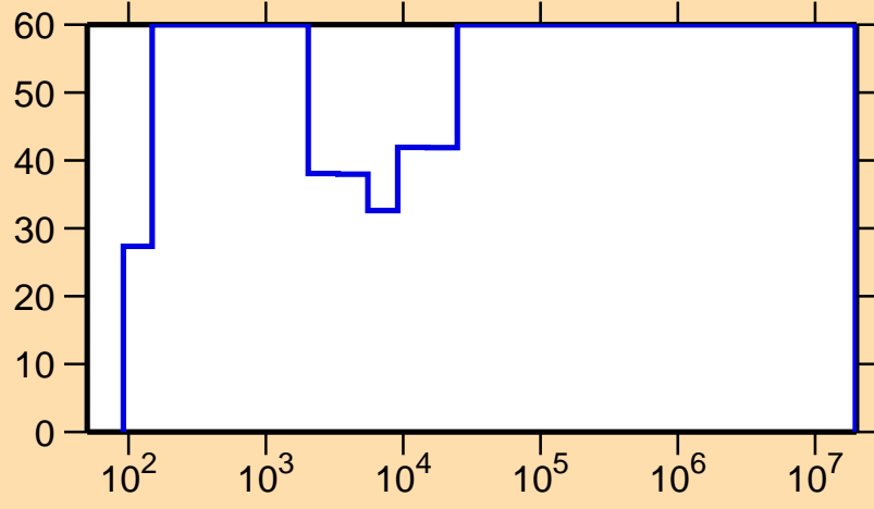
\Delta\sigma/\sigma vs. E for ^{238}\text{Pa}(n,\gamma)
