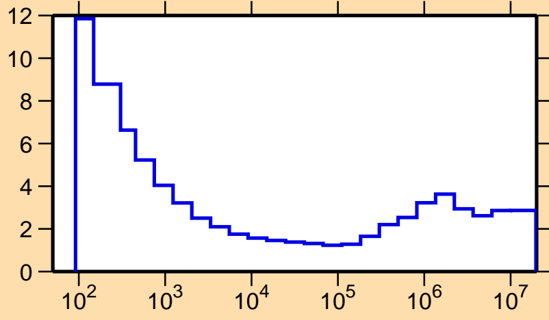
\sigma vs. E for ^{238}\text{Pa}(n,\text{nonel.})
