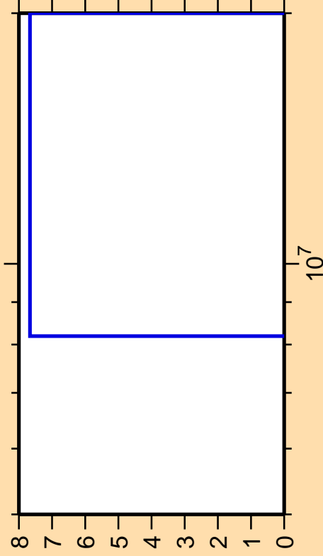
\Delta\sigma/\sigma vs. E for ^{238}\text{Pa}(n,3n\alpha)
