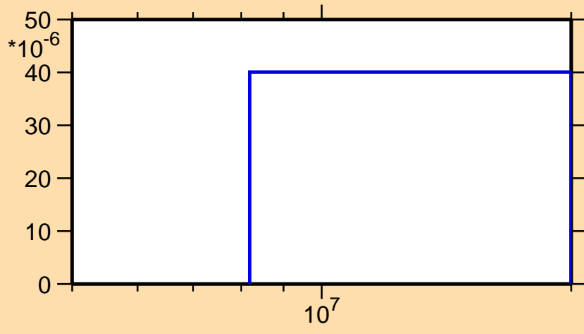
\sigma vs. E for ^{238}\text{Pa}(n,np)
