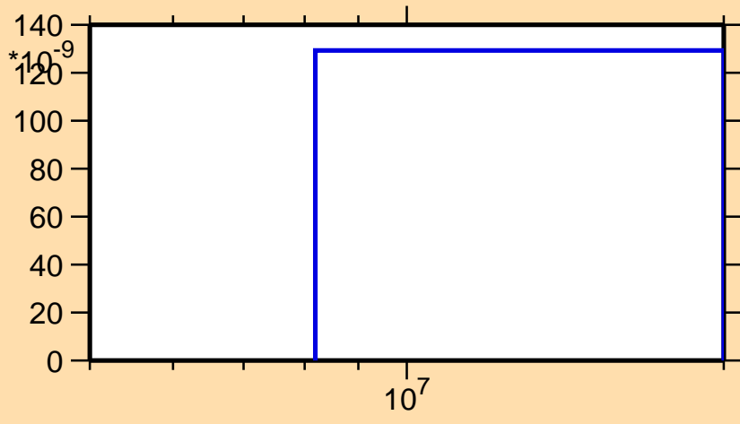
\sigma vs. E for ^{238}\text{Pa}(n,\text{nd})
