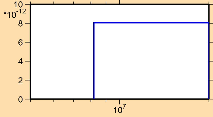
\sigma vs. E for ^{238}\text{Pa}(n,3n\alpha)
