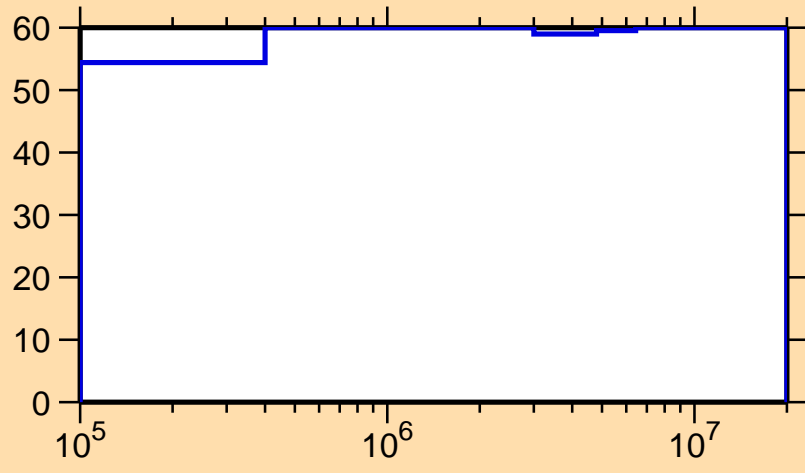
\Delta\sigma/\sigma vs. E for ^{238}\text{Pa}(n,n\text{cont.})
