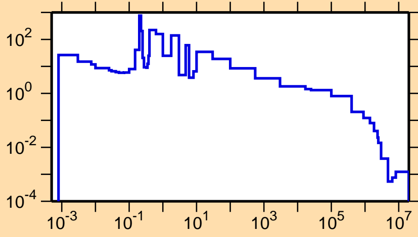
\sigma vs. E for ^{238}\text{Pa}(n,\gamma)
