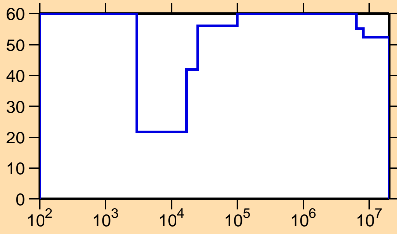
\Delta\sigma/\sigma vs. E for ^{238}\text{Pa}(n,\text{nonel.})
