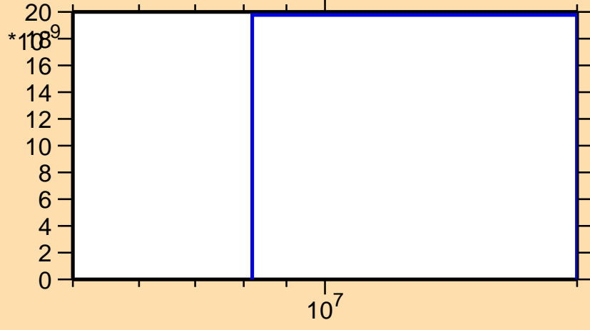
\sigma vs. E for ^{238}\text{Pa}(n,2np)
