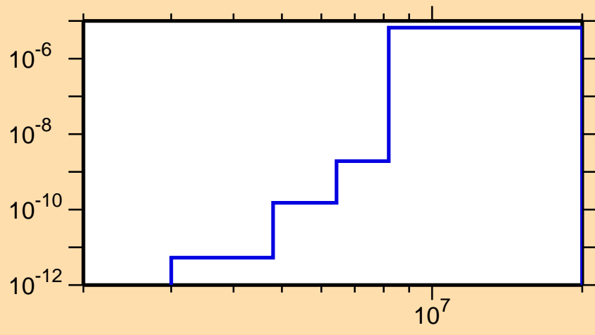
\sigma vs. E for ^{238}\text{Pa}(n,n\alpha)
