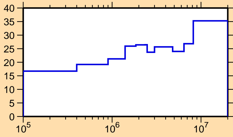
\Delta\sigma/\sigma vs. E for ^{238}\text{Pa}(n,\text{tot.})
