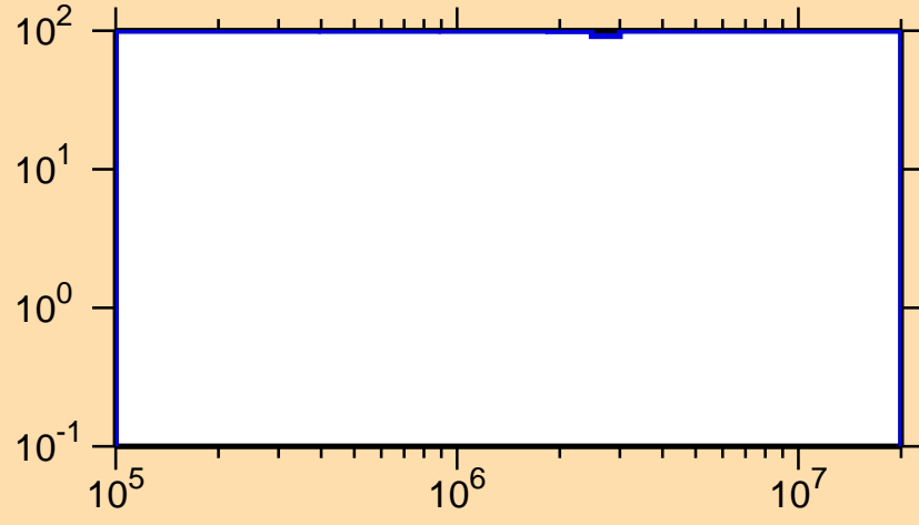
\Delta\sigma/\sigma vs. E for ^{238}\text{Pa}(n,n_1)
