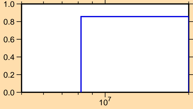
\sigma vs. E for ^{238}\text{Pa}(n,3n)
