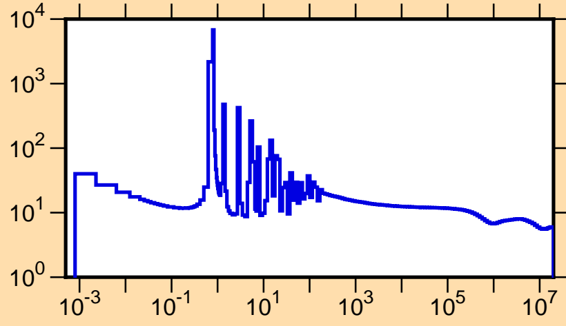
\sigma vs. E for ^{239}\text{Pa}(n,\text{tot.})
