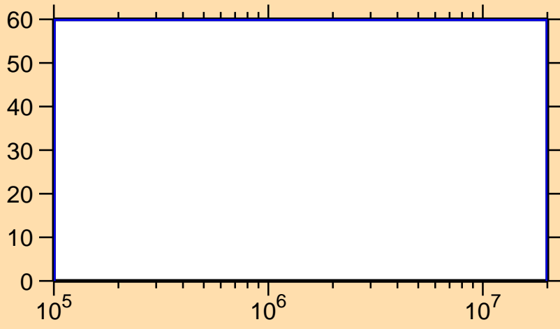
\Delta\sigma/\sigma vs. E for ^{239}\text{Pa}(n,n\text{cont.})
