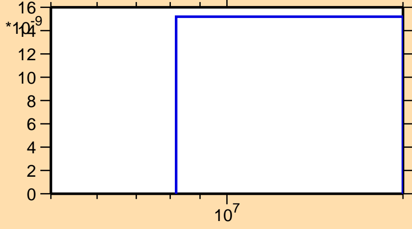
\sigma vs. E for ^{239}\text{Pa}(n,\text{nd})
