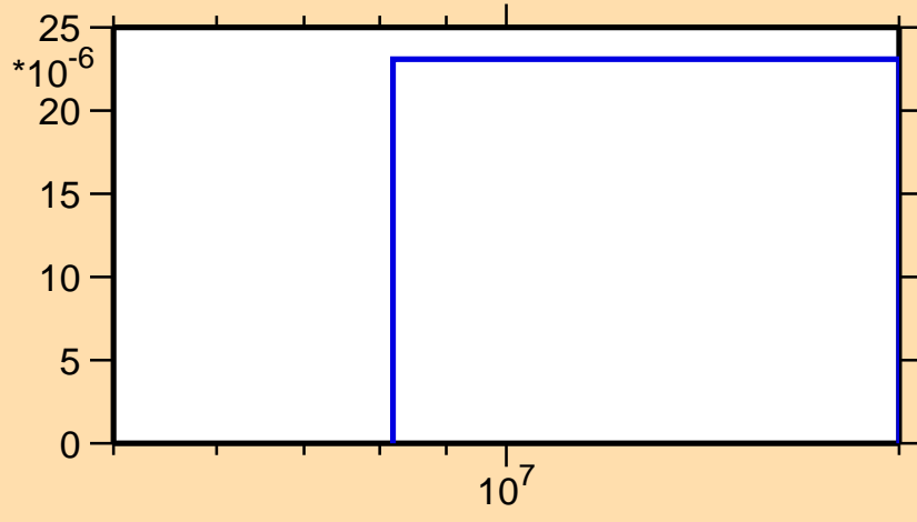
\sigma vs. E for ^{239}\text{Pa}(n,t)
