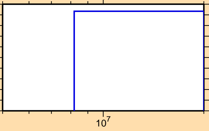
\sigma vs. E for ^{239}\text{Pa}(n,2np)
