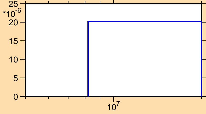
\sigma vs. E for ^{239}\text{Pa}(n,np)
