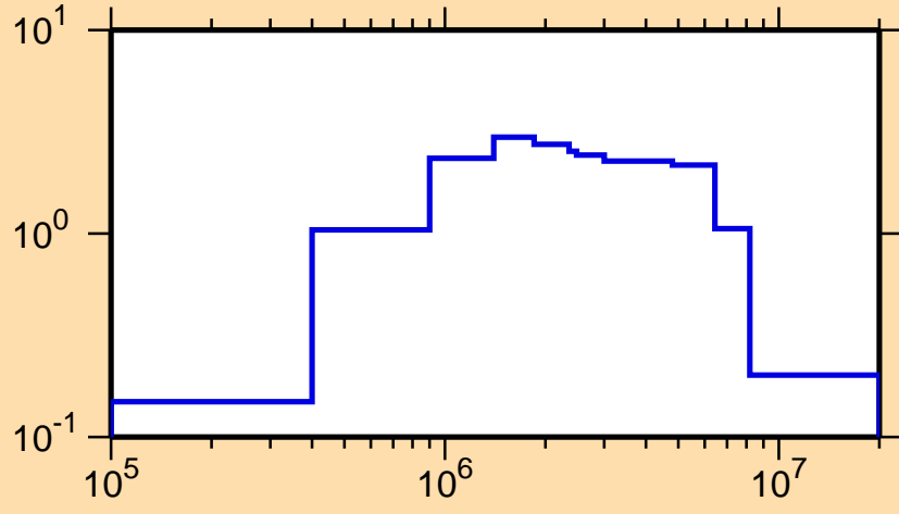
\sigma vs. E for ^{239}\text{Pa}(n,\text{inel.})
