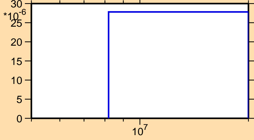
\sigma vs. E for ^{239}\text{Pa}(n,d)
