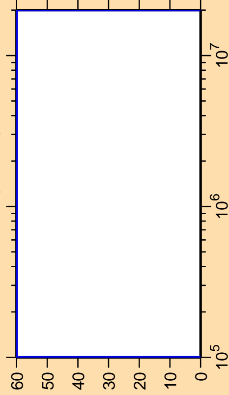
\Delta\sigma/\sigma vs. E for ^{239}\text{Pa}(n,\text{inel.})
