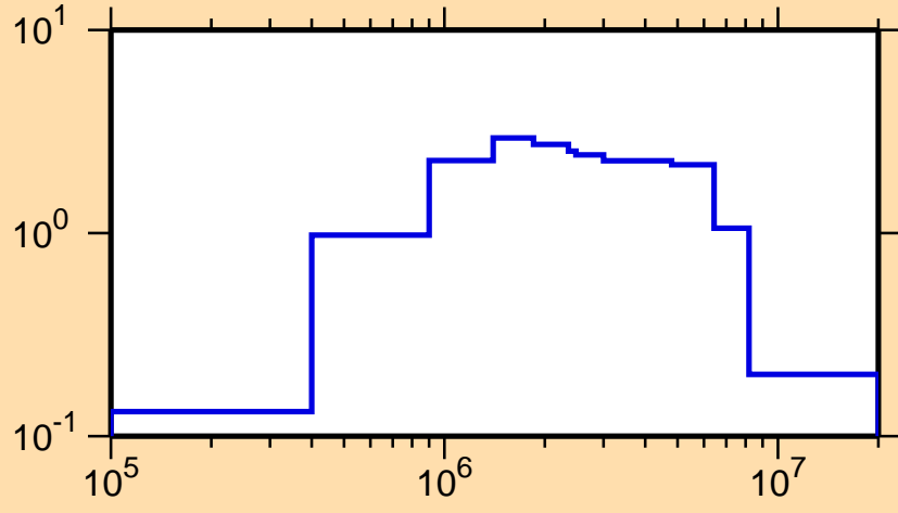
\sigma vs. E for ^{239}\text{Pa}(n,n\text{cont.})
