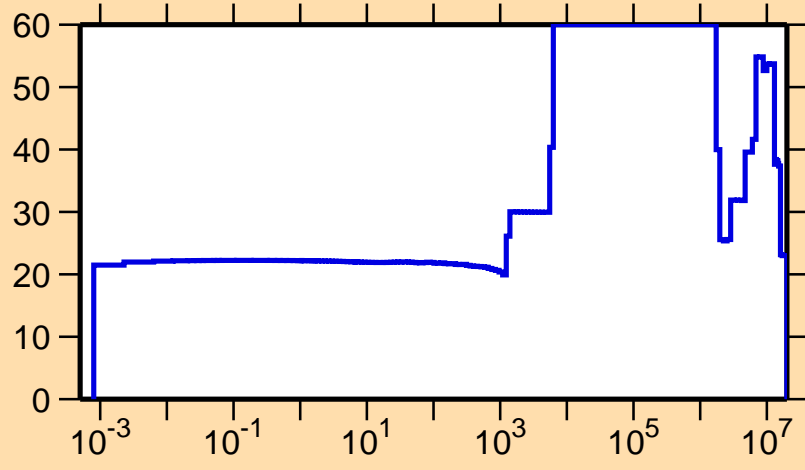
\Delta\sigma/\sigma vs. E for ^{240}\text{Pa}(n,el.)
