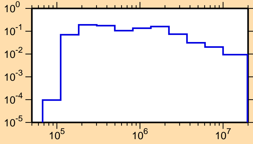
\sigma vs. E for ^{240}\text{Pa}(n,n_1)
