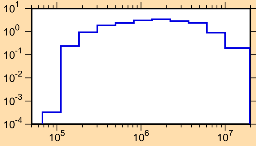
\sigma vs. E for ^{240}\text{Pa}(n,n\text{cont.})
