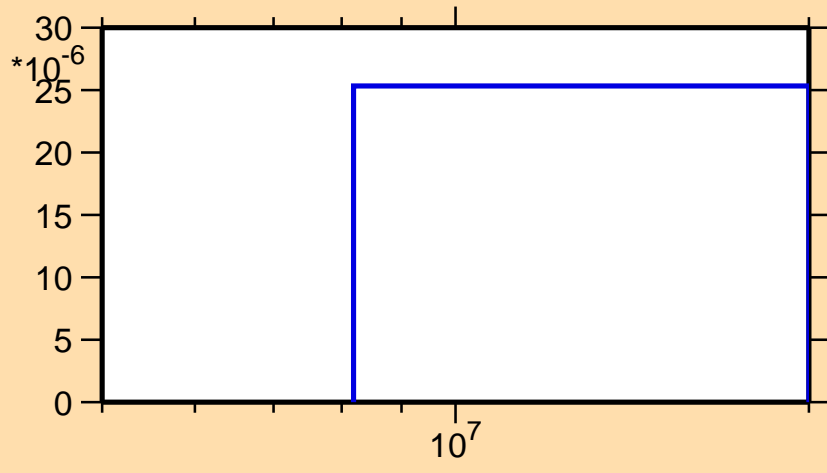
\sigma vs. E for ^{240}\text{Pa}(n,t)
