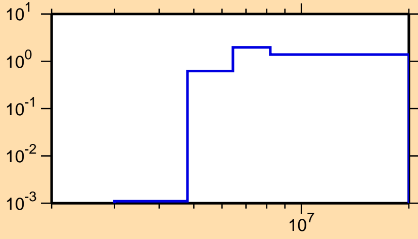
\sigma vs. E for ^{240}\text{Pa}(n,2n)
