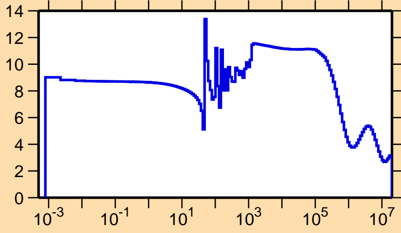
\sigma vs. E for ^{241}\text{Pa}(n,\text{el.})
