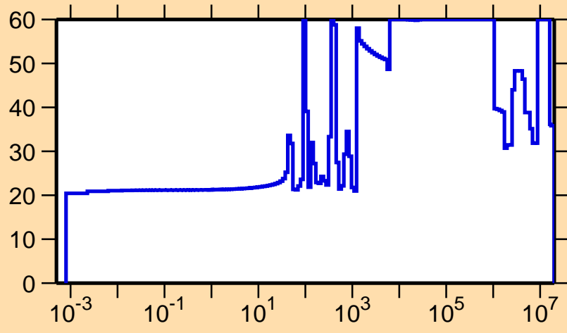
\Delta\sigma/\sigma vs. E for ^{241}\text{Pa}(n,el.)
