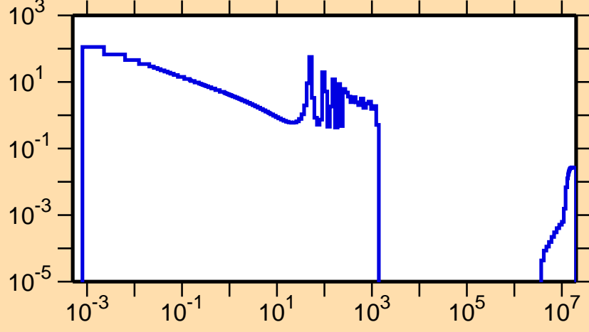
\sigma vs. E for ^{241}\text{Pa}(n,f)
