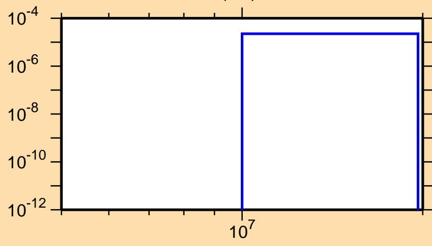
\sigma vs. E for ^{241}\text{Pa}(n,t)
