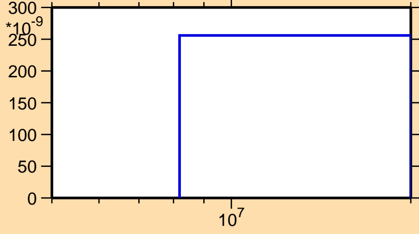
\sigma vs. E for ^{241}\text{Pa}(n,nt)
