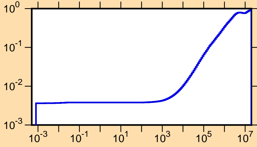
\mu vs. E for ^{186}\text{Pb}(\text{mt251})
