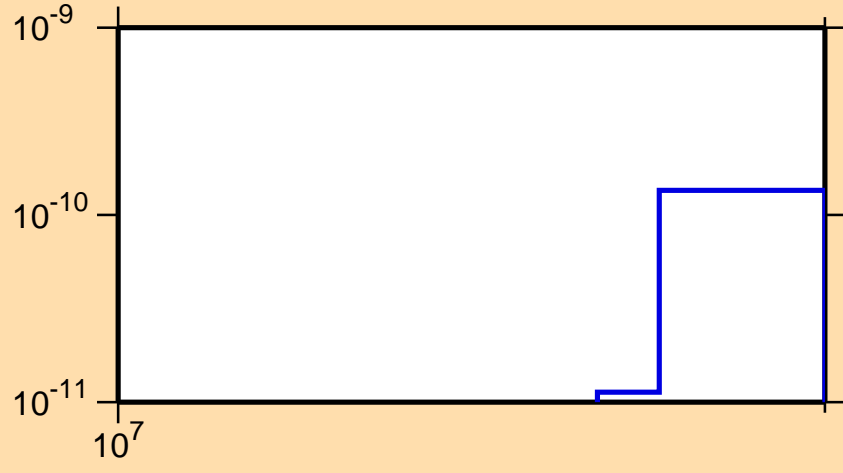
\sigma vs. E for ^{186}\text{Pb} (mt 34)
