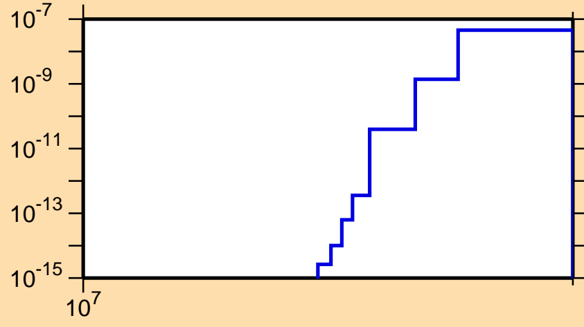
\sigma vs. E for ^{186}\text{Pb}(n,\text{nd})
