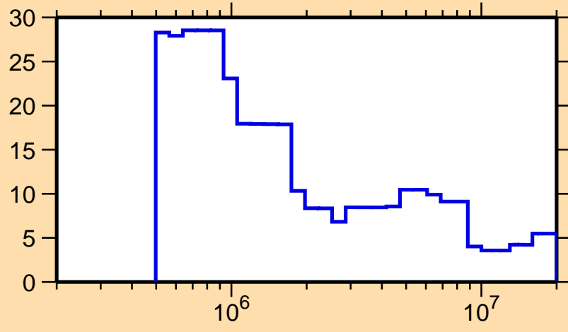
\Delta\sigma/\sigma vs. E for ^{186}\text{Pb}(n,\text{tot.})
