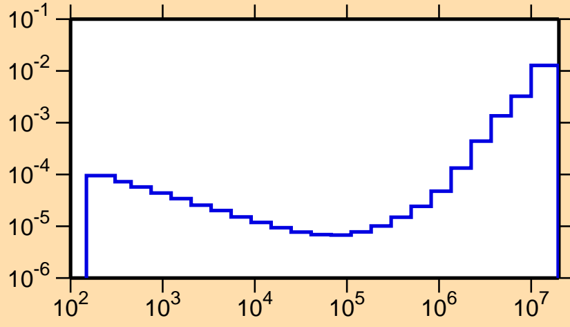
\sigma vs. E for ^{186}\text{Pb}(n,p\alpha)
