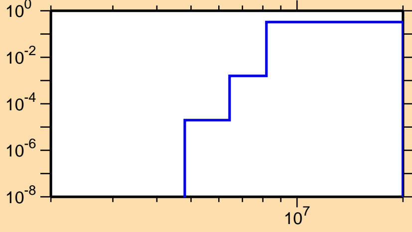
\sigma vs. E for ^{186}\text{Pb}(n,np)
