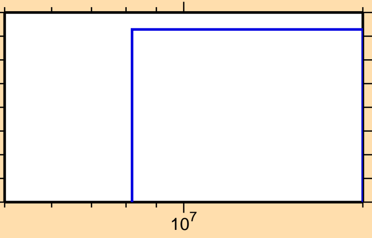
\sigma vs. E for ^{186}\text{Pb}(n,t)
