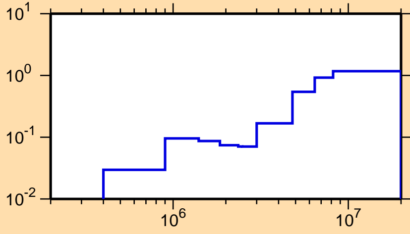
\sigma vs. E for ^{186}\text{Pb}(n,\text{inel.})
