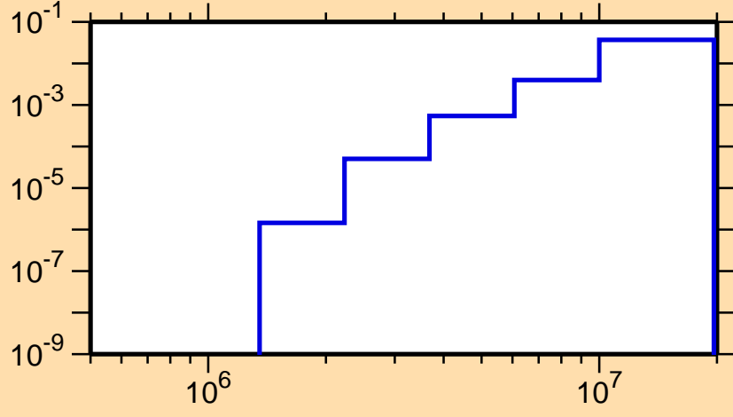
\sigma vs. E for ^{187}\text{Pb}(n,n\alpha)
