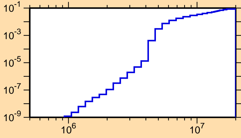
\sigma vs. E for ^{188}\text{Pb}(n,n\alpha)
