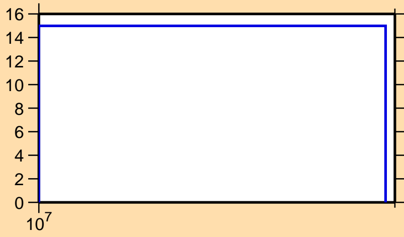
\Delta\sigma/\sigma vs. E for ^{188}\text{Pb}(n,\text{nonel.})
