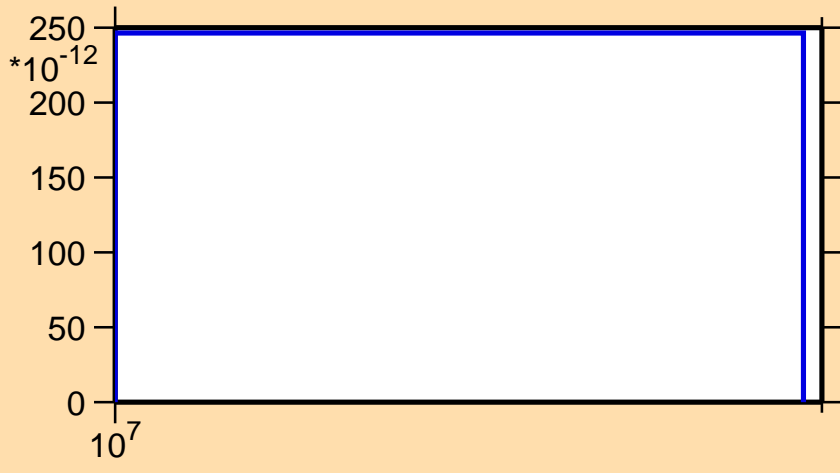
\sigma vs. E for ^{188}\text{Pb}(n,\text{nd})
