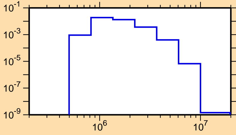
\sigma vs. E for ^{188}\text{Pb}(n,n_4)
