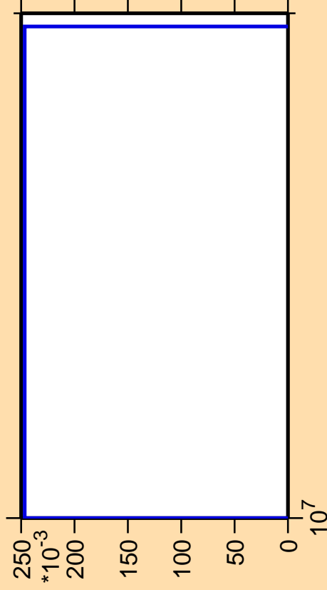
\Delta\sigma/\sigma vs. E for ^{188}\text{Pb}(n,nt)
