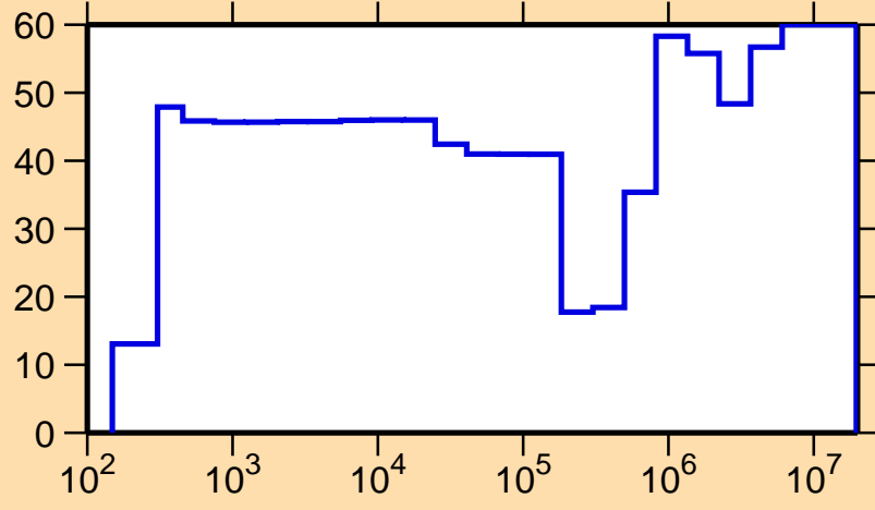
\Delta\sigma/\sigma vs. E for ^{188}\text{Pb}(n,\text{el.})
