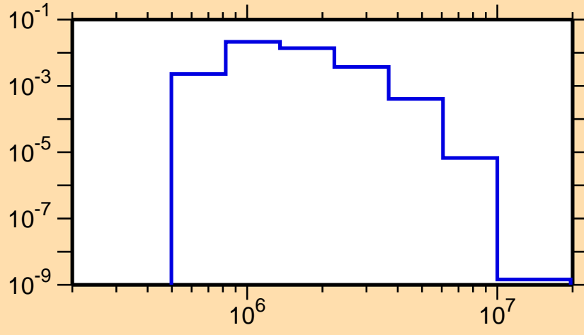
\sigma vs. E for ^{188}\text{Pb}(n,n_3)
