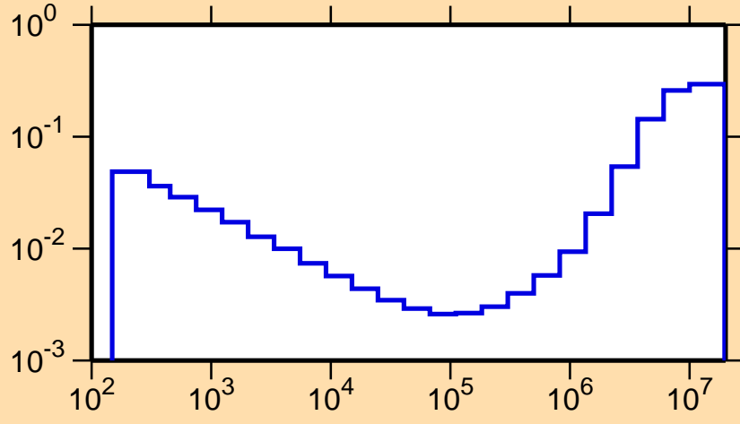
\sigma vs. E for ^{188}\text{Pb}(n,p)
