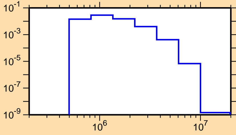
\sigma vs. E for ^{188}\text{Pb}(n,n_1)
