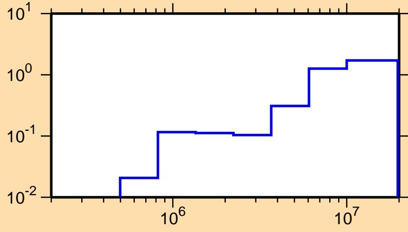
\sigma vs. E for ^{188}\text{Pb}(n,\text{inel.})
