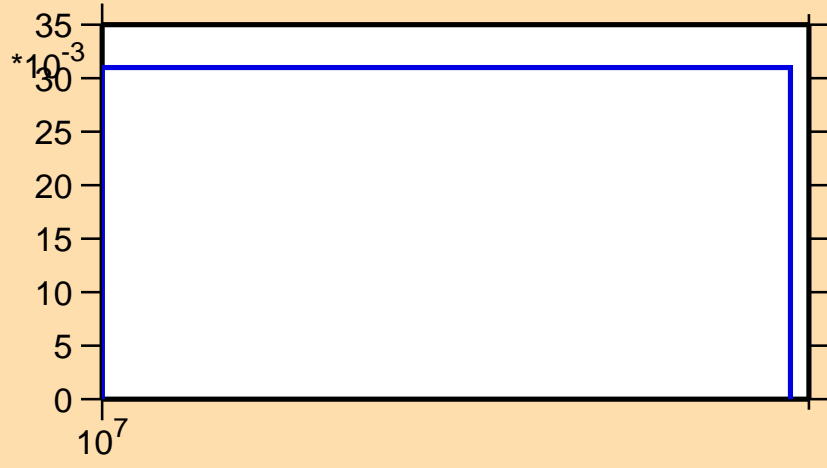
\sigma vs. E for ^{188}\text{Pb}(n,2n)
