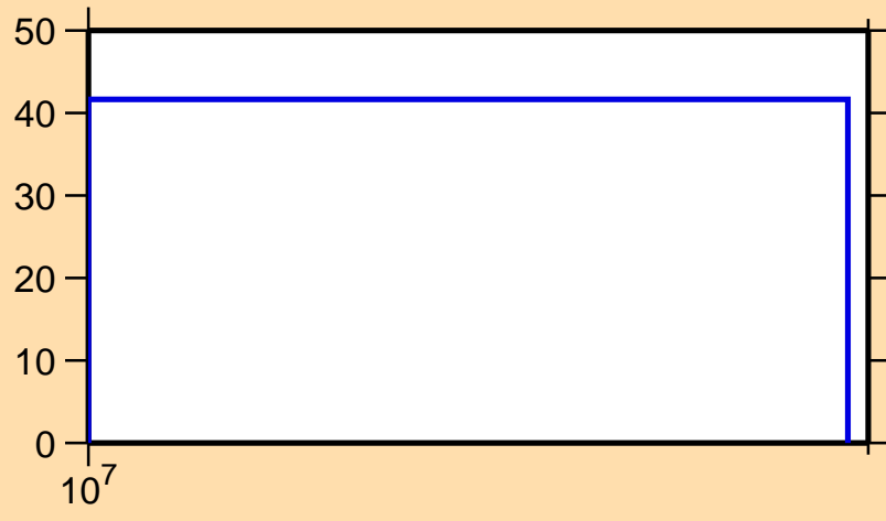
\Delta\sigma/\sigma vs. E for ^{188}\text{Pb}(n,\text{tot.})
