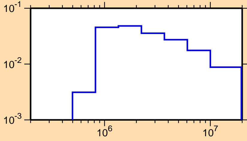
\sigma vs. E for ^{188}\text{Pb}(n,n_2)
