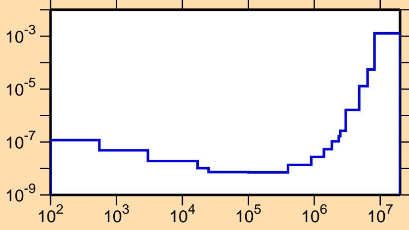
\sigma vs. E for ^{188}\text{Pb}(n,p\alpha)
