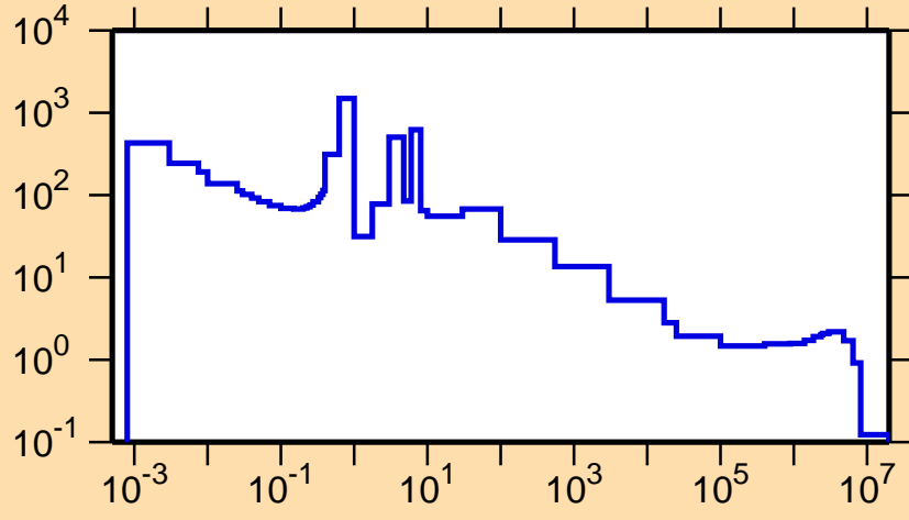
\sigma vs. E for ^{188}\text{Pb}(n,\gamma)
