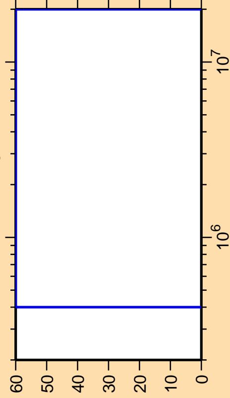
\Delta\sigma/\sigma vs. E for ^{188}\text{Pb}(n,n_3)
