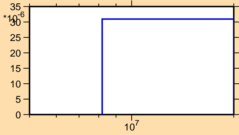
\sigma vs. E for ^{188}\text{Pb}(n,t)
