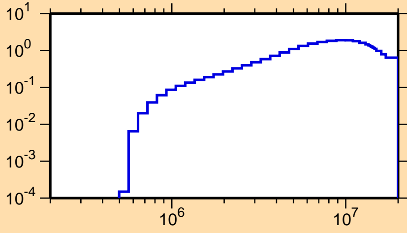
\sigma vs. E for ^{189}\text{Pb}(n,\text{inel.})
