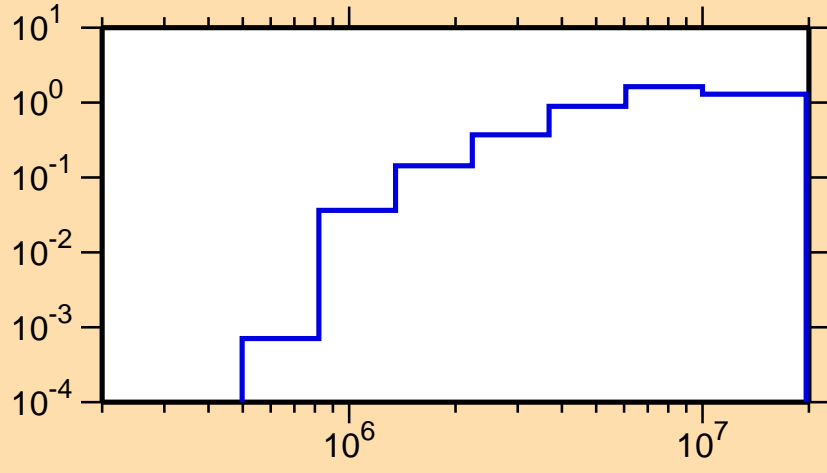
\sigma vs. E for ^{189}\text{Pb}(n,n\text{cont.})
