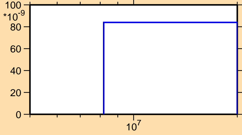
\sigma vs. E for ^{189}\text{Pb}(n,\text{nd})
