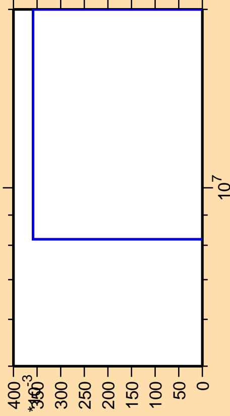
\Delta\sigma/\sigma vs. E for ^{190}\text{Pb}(\text{mt } 34)
