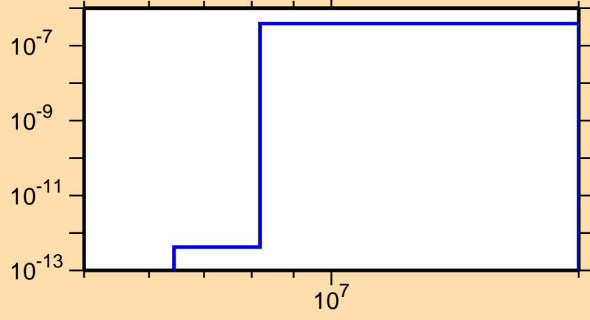
\sigma vs. E for ^{190}\text{Pb}(n,\text{He}3)
