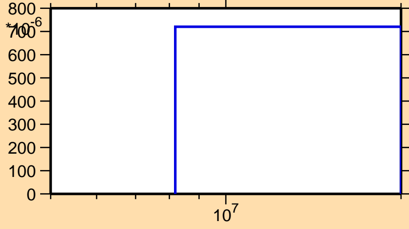
\sigma vs. E for ^{190}\text{Pb}(n,2n\alpha)
