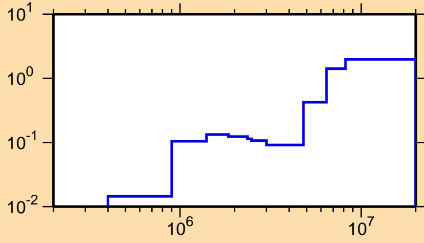
\sigma vs. E for ^{190}\text{Pb}(n,\text{inel.})
