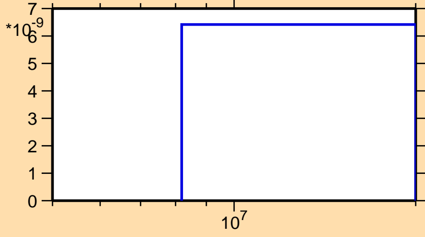
\sigma vs. E for ^{190}\text{Pb}(n,\text{pd})
