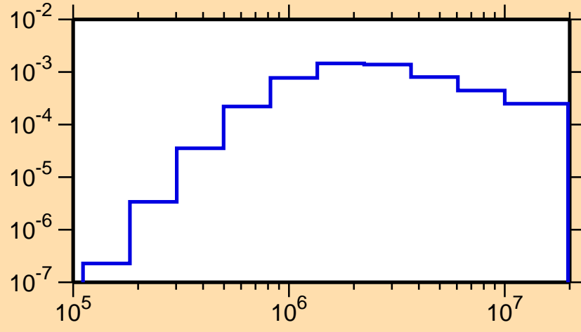
\sigma vs. E for ^{191}\text{Pb}(n,n_1)
