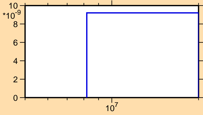
\sigma vs. E for ^{191}\text{Pb}(n,\text{pd})
