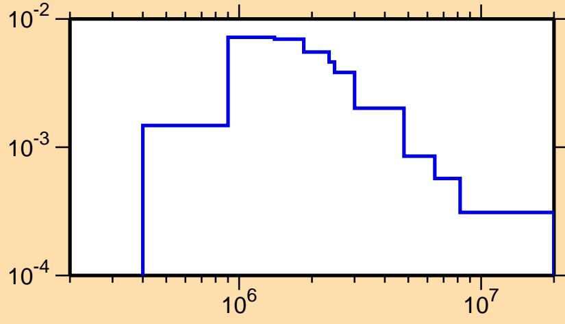
\sigma vs. E for ^{191}\text{Pb}(n,n_3)
