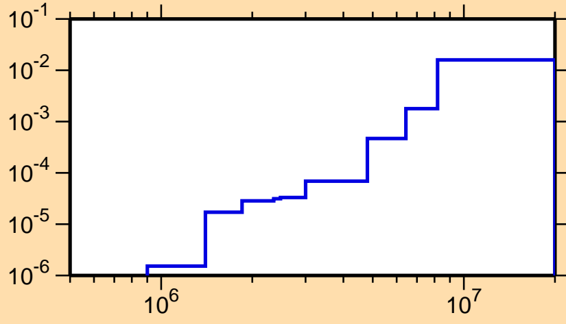
\sigma vs. E for ^{191}\text{Pb}(n,n\alpha)
