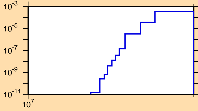
\sigma vs. E for ^{191}\text{Pb}(n,2np)
