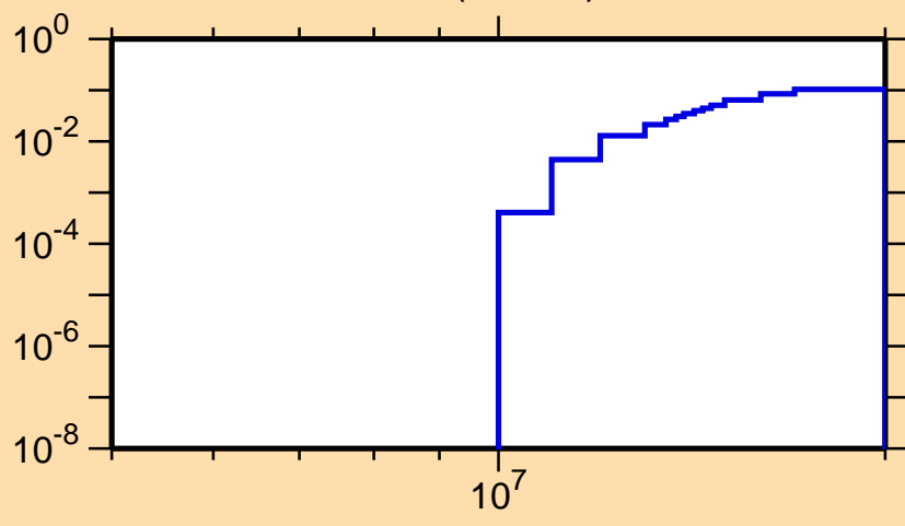
\sigma vs. E for ^{191}\text{Pb}(n,2n\alpha)
