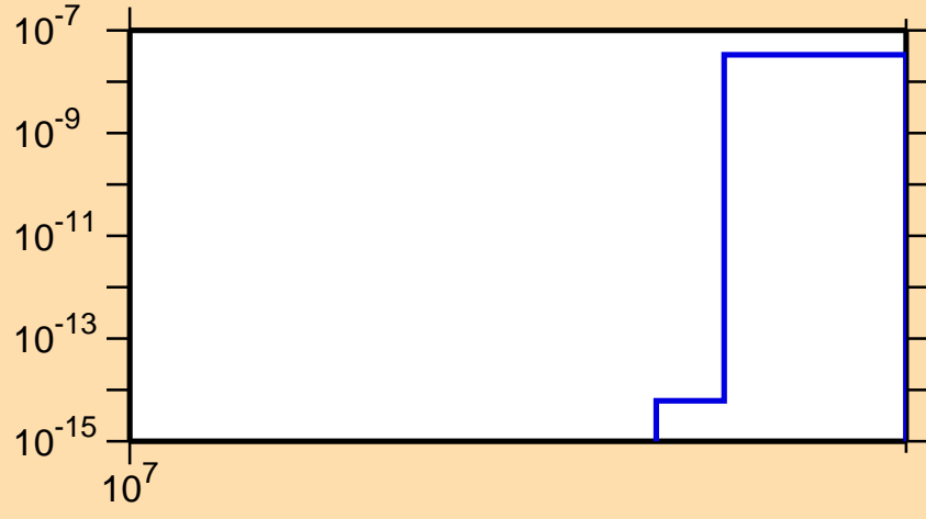
\sigma vs. E for ^{191}\text{Pb}(n,3n\alpha)
