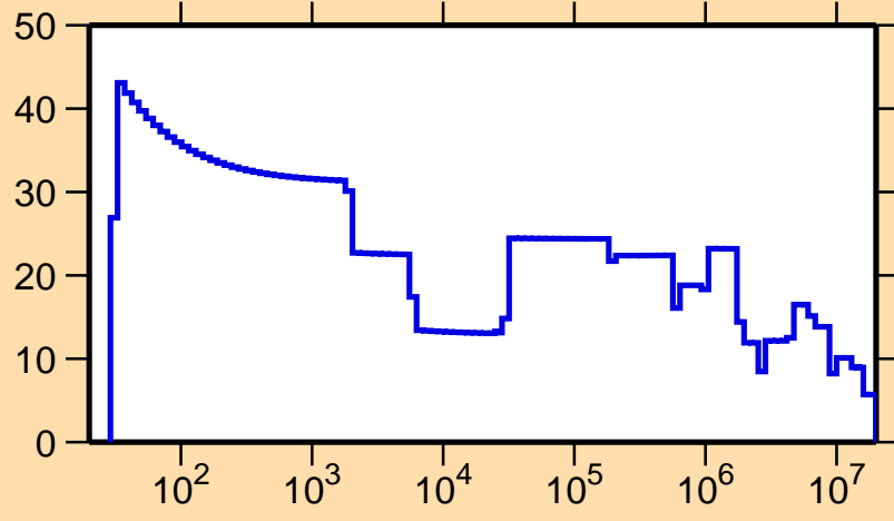
\Delta\sigma/\sigma vs. E for ^{191}\text{Pb}(n,\text{el.})
