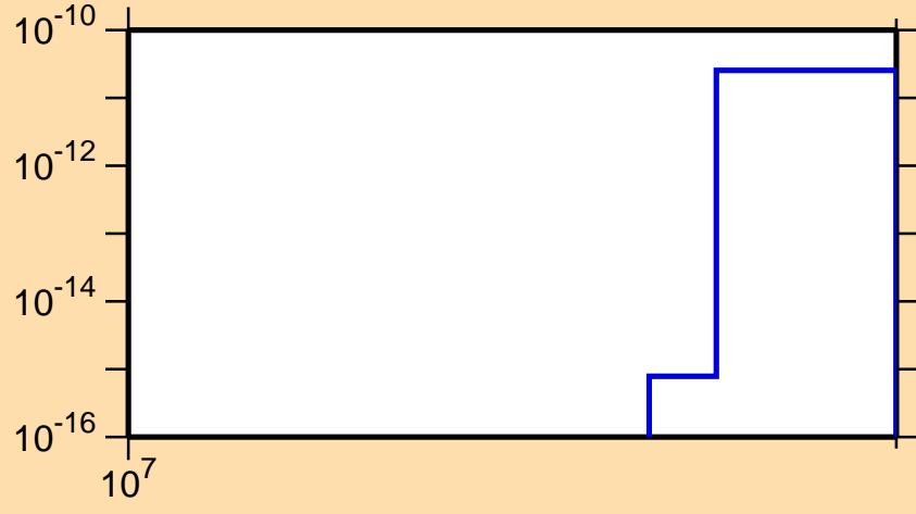
\sigma vs. E for ^{191}\text{Pb}(n,nt)
