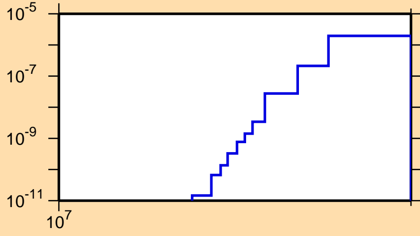
\sigma vs. E for ^{191}\text{Pb}(n,\text{nd})
