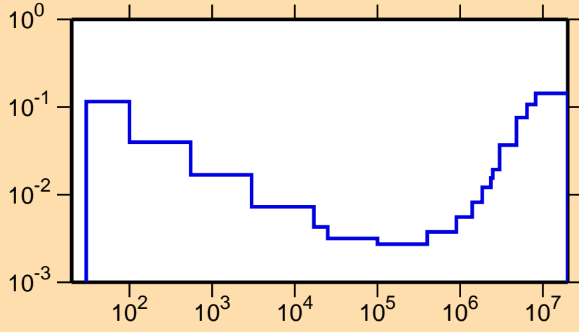
\sigma vs. E for ^{191}\text{Pb}(n,p)
