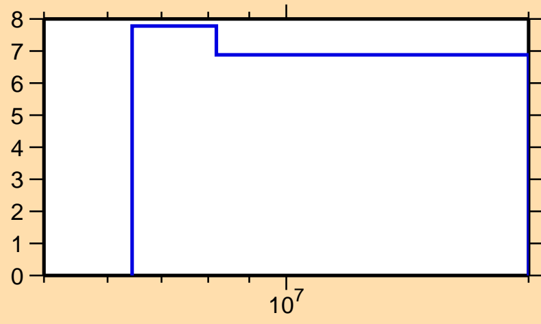
\Delta\sigma/\sigma vs. E for ^{191}\text{Pb}(n,\text{nonel.})
