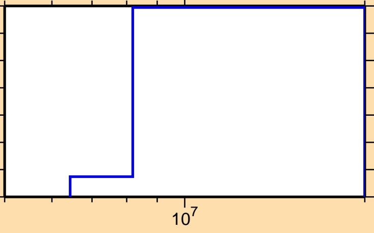
\sigma vs. E for ^{191}\text{Pb}(n,\text{He3})
