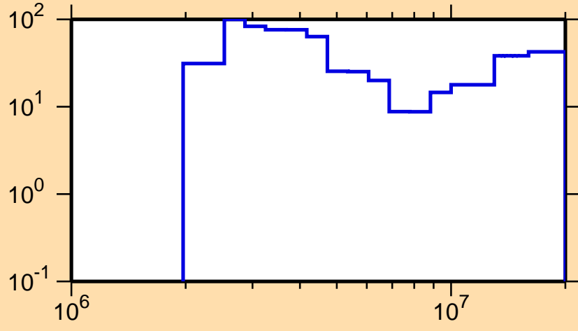
\Delta\sigma/\sigma vs. E for ^{192}\text{Pb}(n,n\text{cont.})
