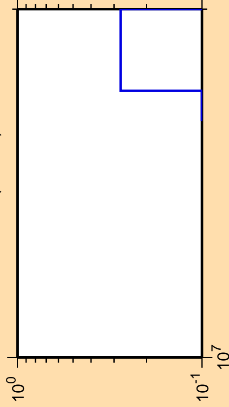
\Delta\sigma/\sigma vs. E for ^{192}\text{Pb}(n,3n\alpha)
