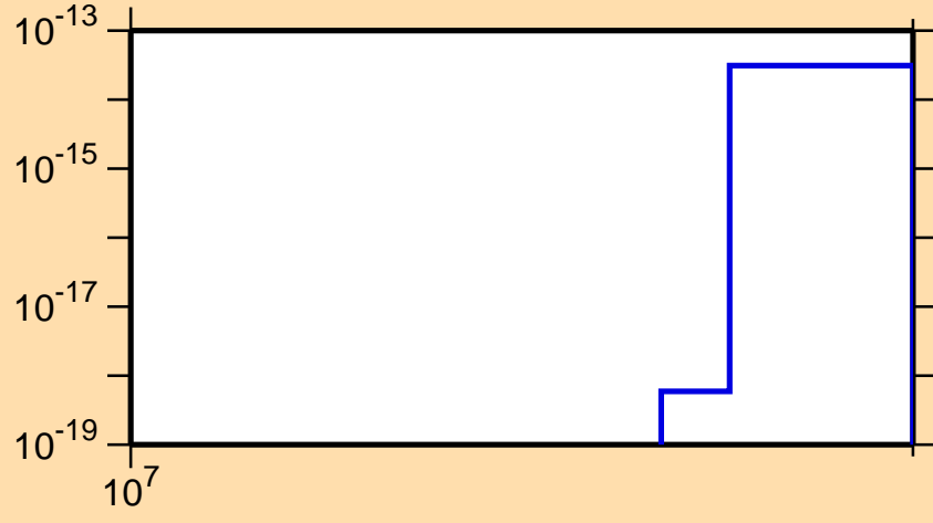
\sigma vs. E for ^{192}\text{Pb}(n,3n\alpha)
