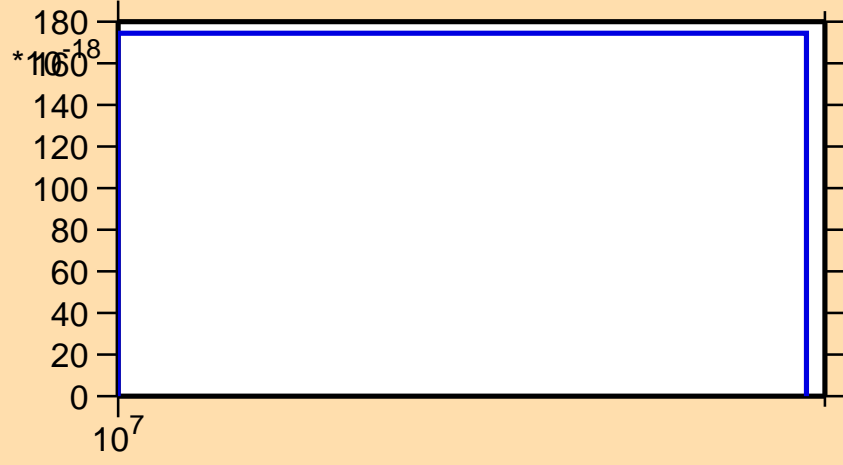
\sigma vs. E for ^{192}\text{Pb}(n,3n\alpha)
