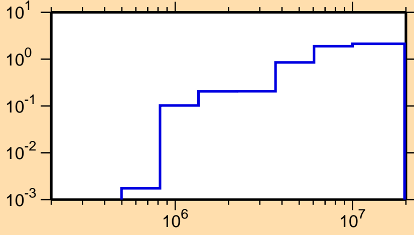
\sigma vs. E for ^{192}\text{Pb}(n,\text{inel.})
