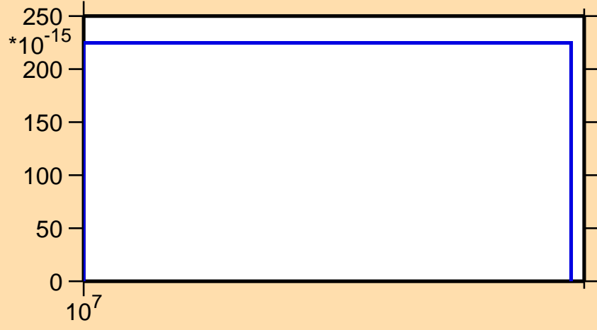
\sigma vs. E for ^{192}\text{Pb}(n,nt)
