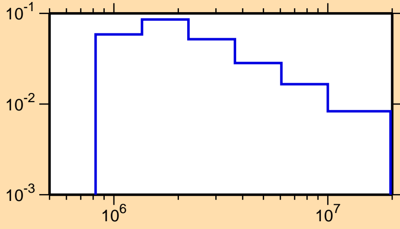
\sigma vs. E for ^{192}\text{Pb}(n,n_2)
