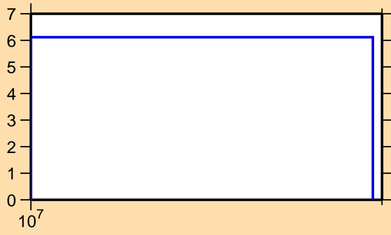
\Delta\sigma/\sigma vs. E for ^{192}\text{Pb}(n,\text{el.})
