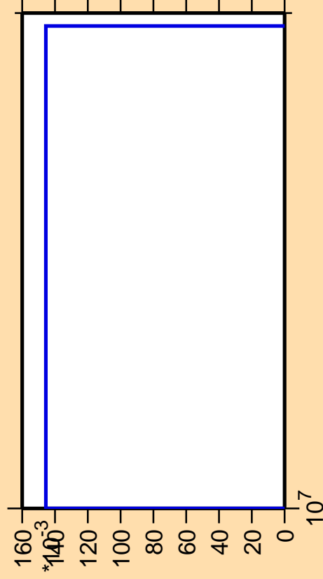
\Delta\sigma/\sigma vs. E for ^{192}\text{Pb}(\text{mt } 34)
