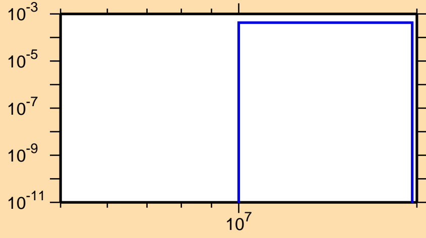
\sigma vs. E for ^{192}\text{Pb}(n,2n\alpha)
