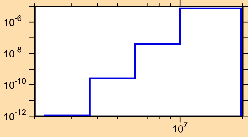
\sigma vs. E for ^{192}\text{Pb}(n,p\alpha)
