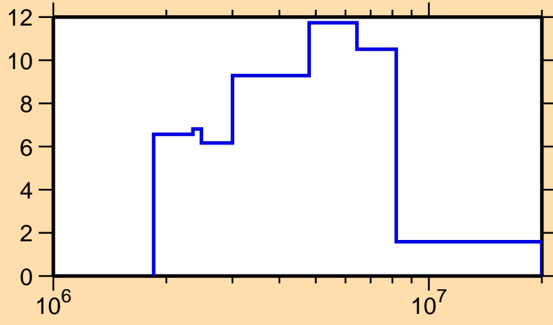
\Delta\sigma/\sigma vs. E for ^{192}\text{Pb}(n, tot.)
