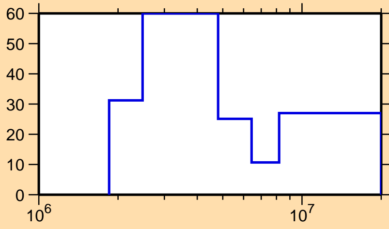
\Delta\sigma/\sigma vs. E for ^{192}\text{Pb}(n,n\text{cont.})
