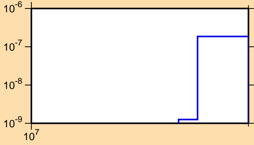
\sigma vs. E for ^{193}\text{Pb}(n,3n\alpha)
