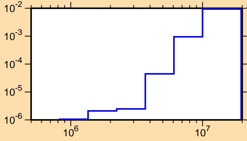
\sigma vs. E for ^{193}\text{Pb}(n,n\alpha)
