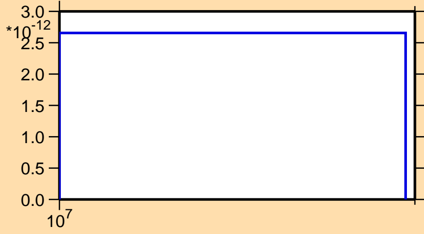
\sigma vs. E for ^{193}\text{Pb} (mt 34)
