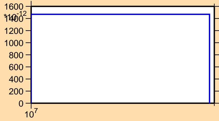
\sigma vs. E for ^{193}\text{Pb}(n,3n\alpha)
