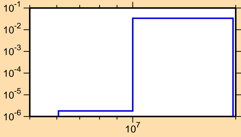
\sigma vs. E for ^{193}\text{Pb}(n,2n\alpha)
