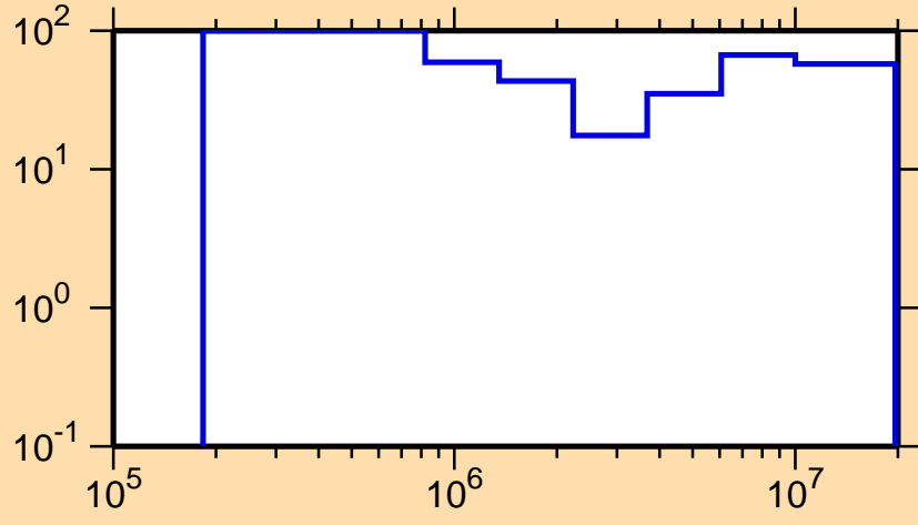
\Delta\sigma/\sigma vs. E for ^{193}\text{Pb}(n,n_1)
