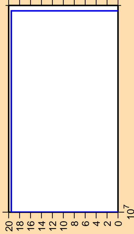
\Delta\sigma/\sigma vs. E for ^{193}\text{Pb} (mt 34)
