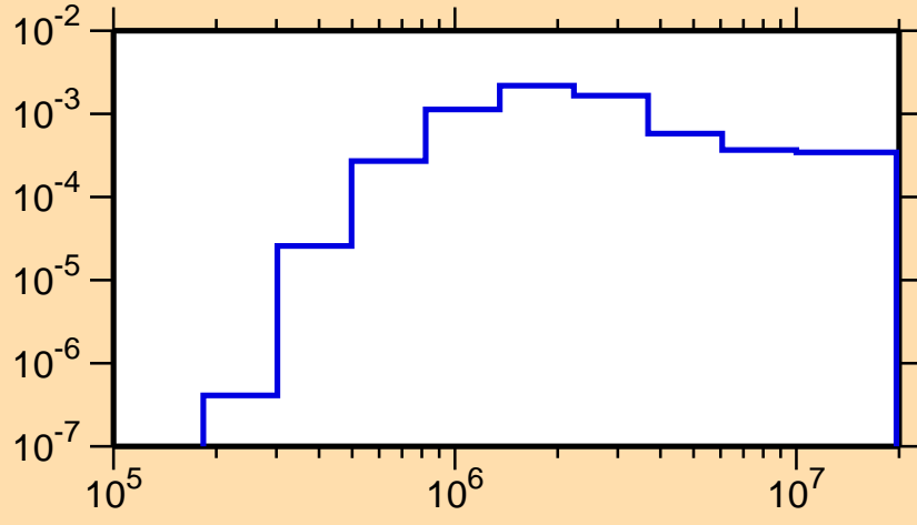
\sigma vs. E for ^{193}\text{Pb}(n,n_1)
