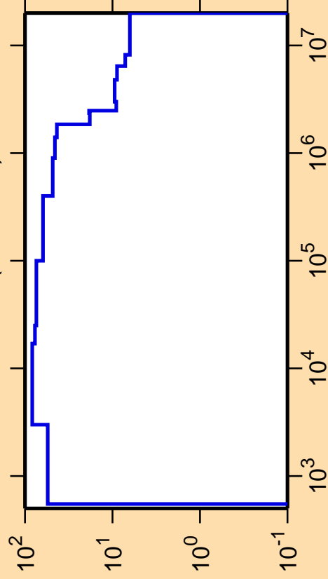
\Delta\sigma/\sigma vs. E for ^{193}\text{Pb}(n,\text{nonel.})
