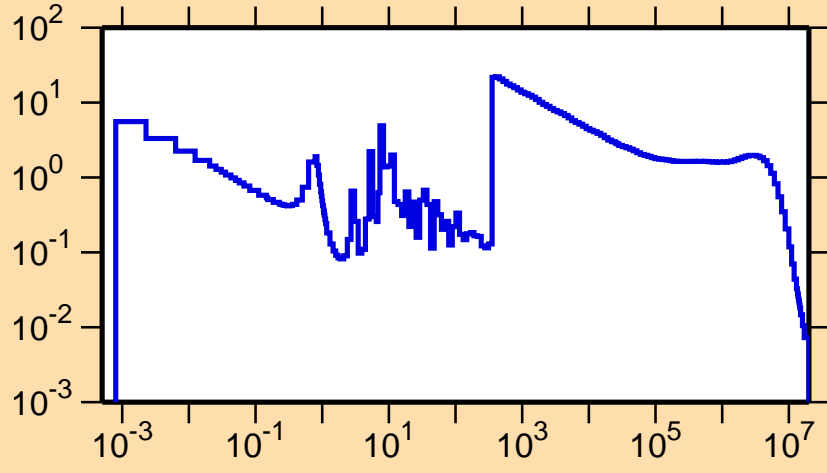
\sigma vs. E for ^{193}\text{Pb}(n,\gamma)
