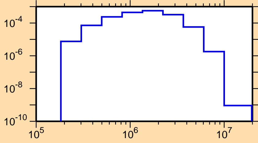
\sigma vs. E for ^{193}\text{Pb}(n,n_2)
