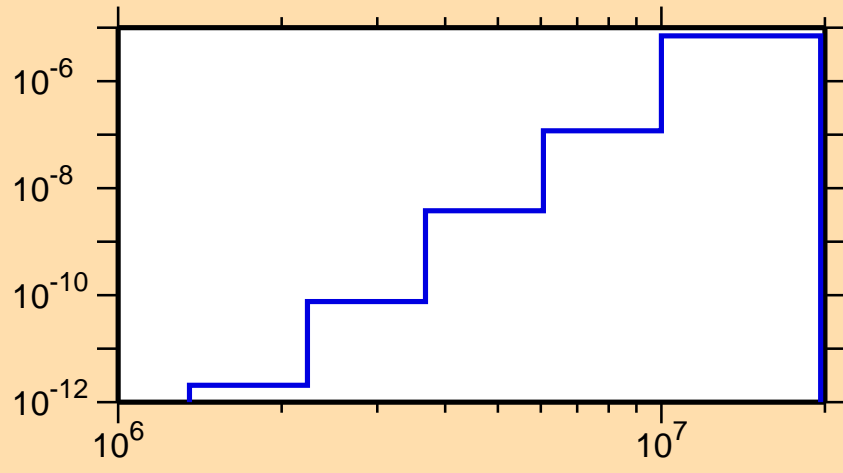
\sigma vs. E for ^{193}\text{Pb}(n,p\alpha)
