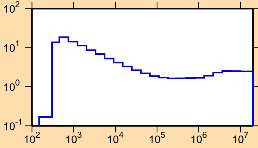
\sigma vs. E for ^{193}\text{Pb}(n,\text{nonel.})
