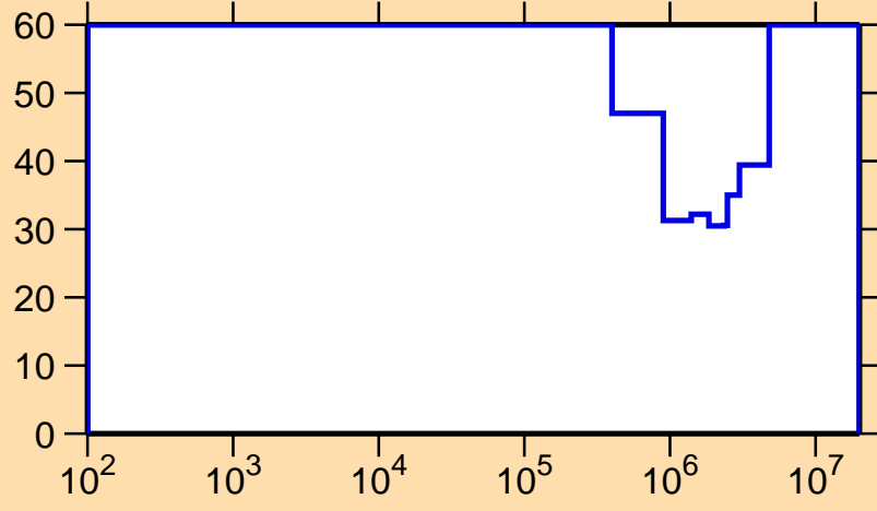
\Delta\sigma/\sigma vs. E for ^{193}\text{Pb}(n,\gamma)
