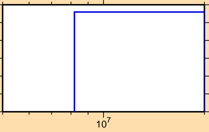
\sigma vs. E for ^{193}\text{Pb}(\text{mt } 45)
