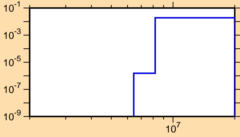
\sigma vs. E for ^{193}\text{Pb}(n,np)
