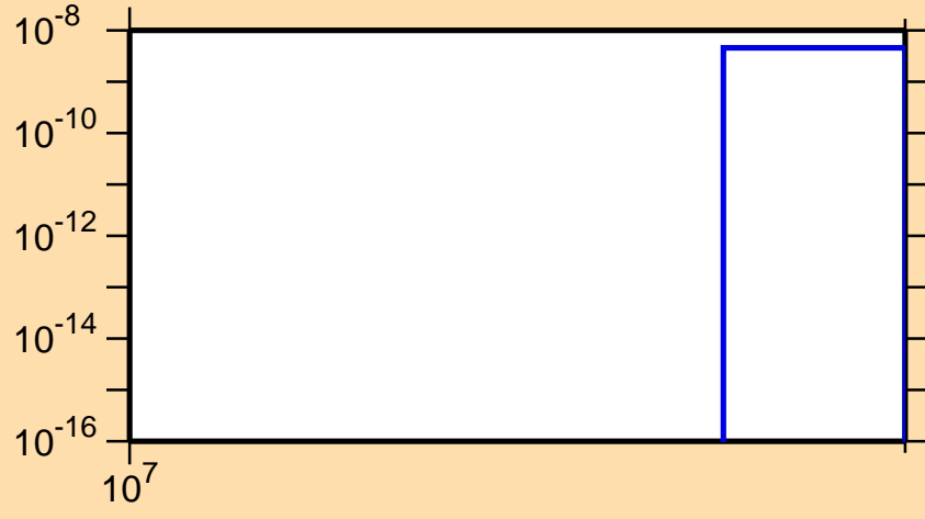
\sigma vs. E for ^{194}\text{Pb}(n,3n\alpha)
