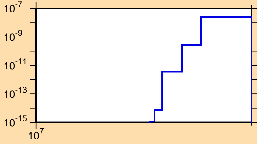
\sigma vs. E for ^{194}\text{Pb}(n,\text{nd})
