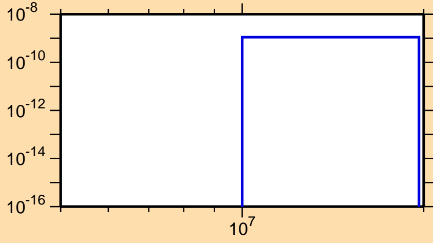
\sigma vs. E for ^{194}\text{Pb}(\text{mt } 45)
