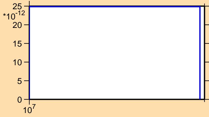
\sigma vs. E for ^{194}\text{Pb}(n,3n\alpha)
