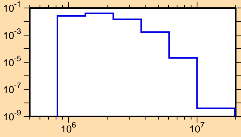
\sigma vs. E for ^{194}\text{Pb}(n,n_1)
