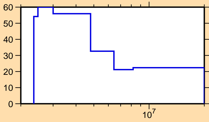
\Delta\sigma/\sigma vs. E for ^{194}\text{Pb}(n,n\text{cont.})
